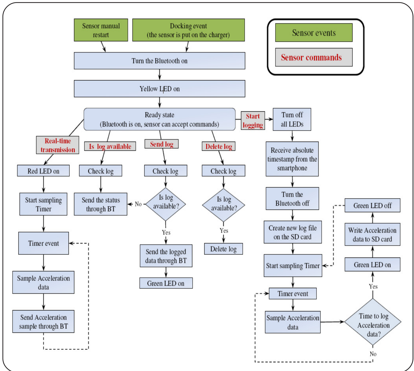
Figure 1. Sensor Firmware Flowchart
