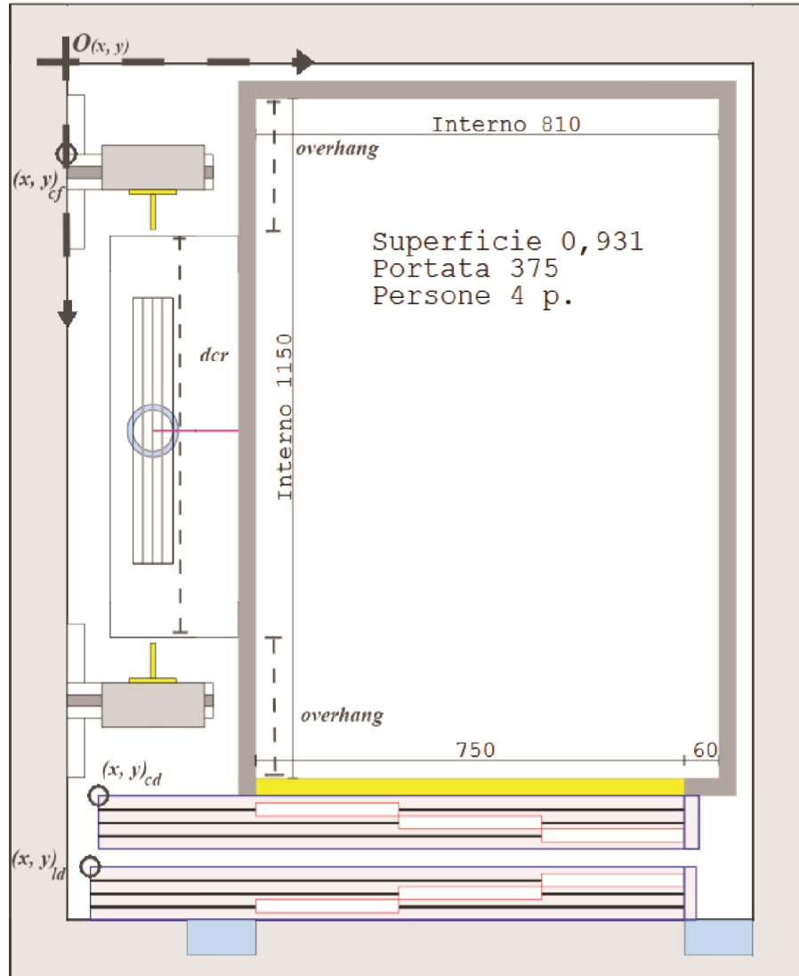
Figure 1. Top view of a configured HE. The shaft is outlined by a gray enclosure in which the components are placed. This elevator has the car frame on the left side and a single door which opens on the bottom of the drawing. The opening area is outlined in the bottom car wall
