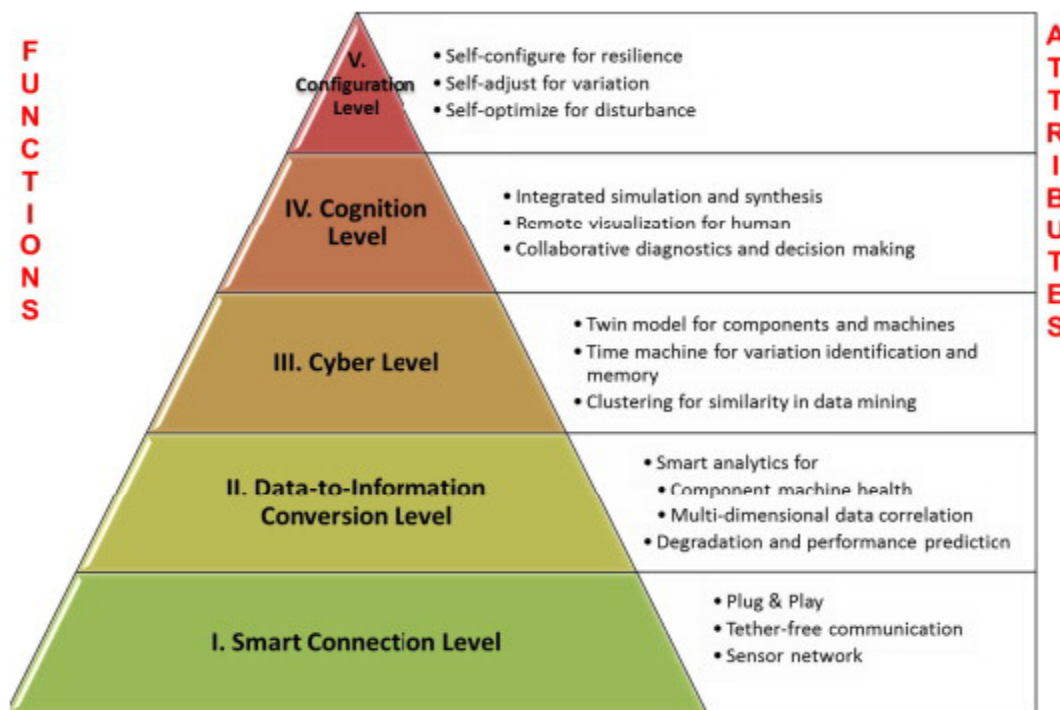
Figure 2. 5C architecture for the implementation of a cyber-physical system [18]
