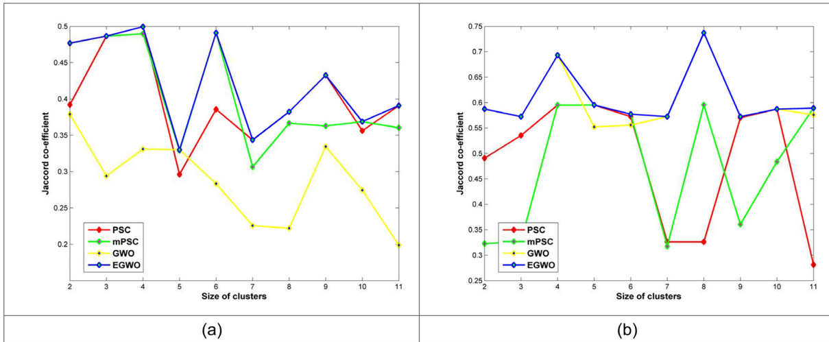
Figure 8. Jaccard coefficient
