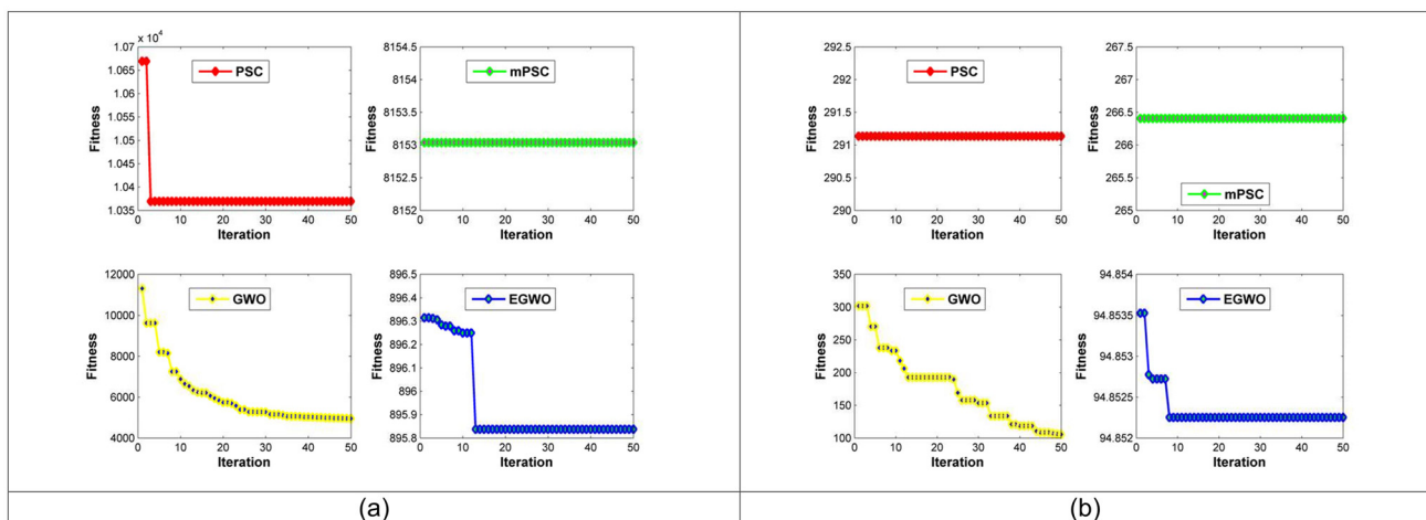
Figure 5. Sum of squared distance
