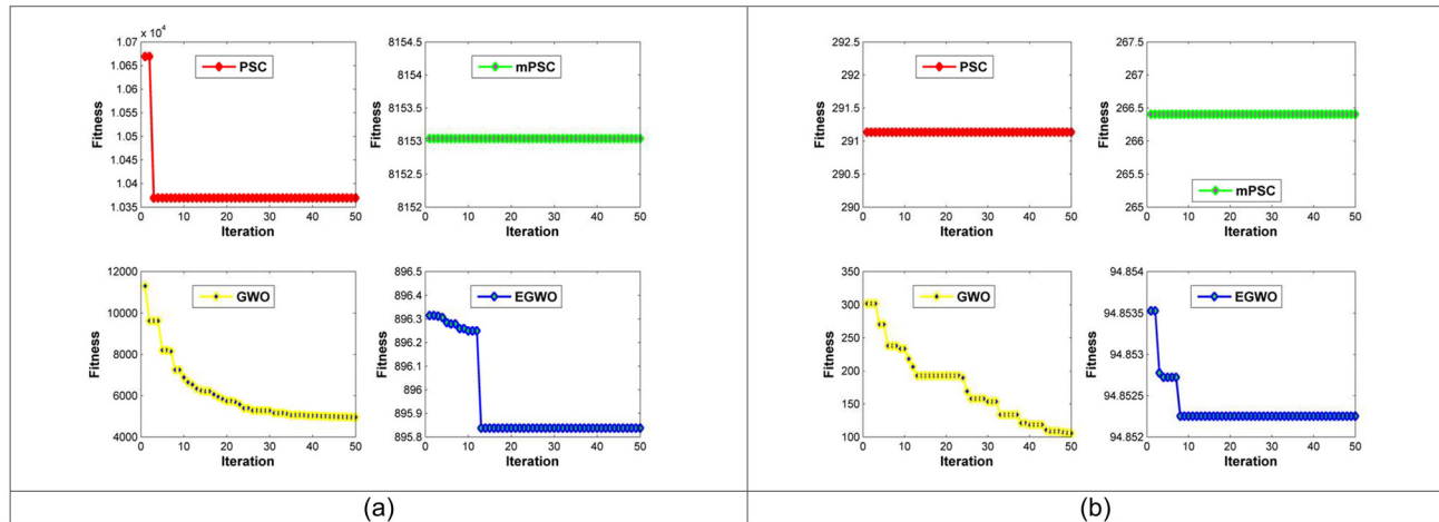
Figure 4. Convergence graph
