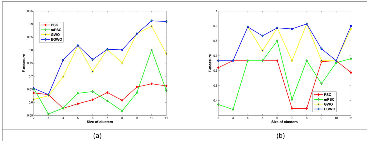
Figure 6. F-measure
