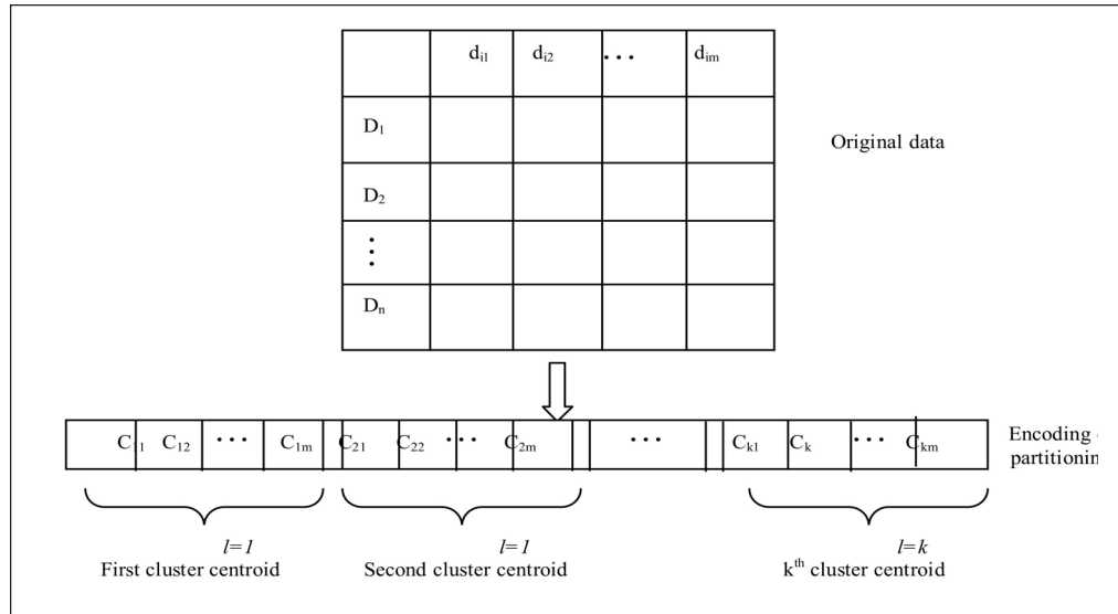
Figure 1. Sample encoding mechanism for KEGWO algorithm
