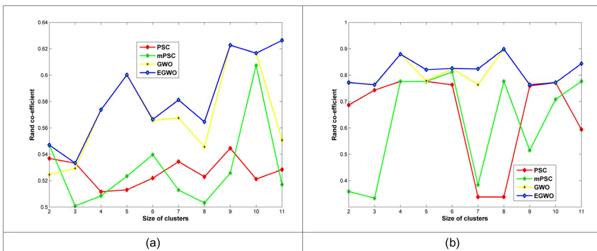
Figure 7. Rand coefficient
