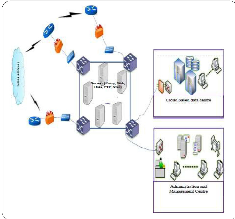
Figure 4. Architecture for IoT Based Information Kendra
