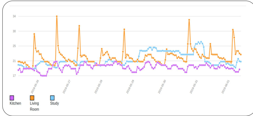
(b) Seven-day test observed from the Temperature sensor
