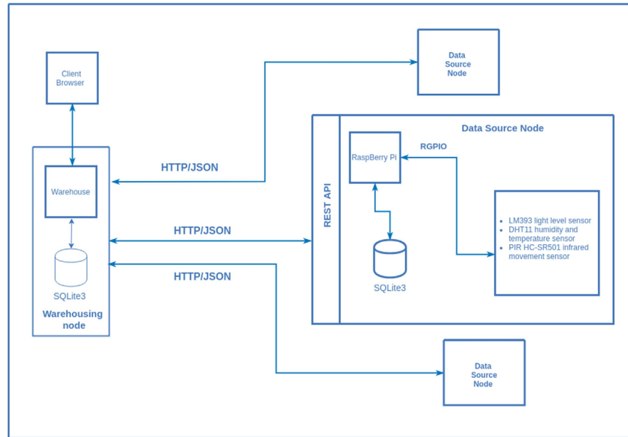
Figure 2. Specific architecture hardware design, applied to the proof of concept
