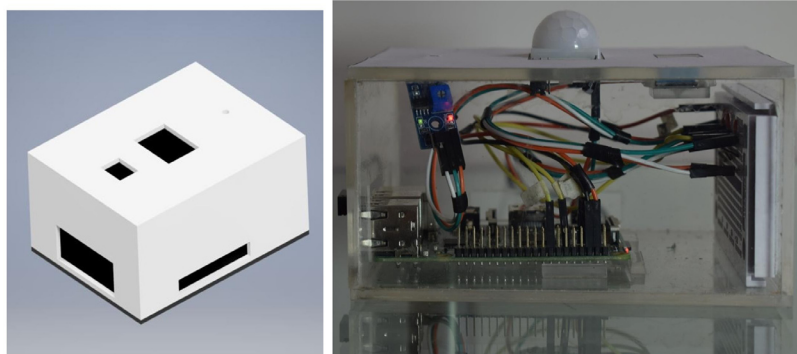
Figure 8. This is the box that was designed for the sensor
