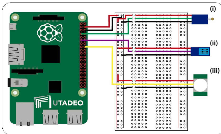
Figure 3. Node hardware design, showing sensors connected to Raspberry Pi B+
