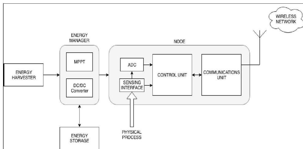
Figure 1. Generic Energy Harvesting WSN Node
