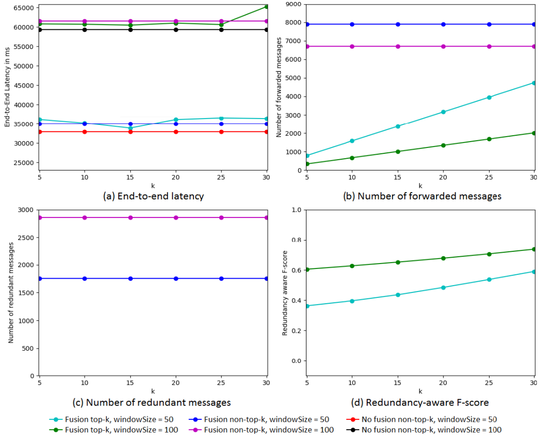
Figure 4. Evaluation results for 50 publishers and 1 subscriber with 50 subscriptions
