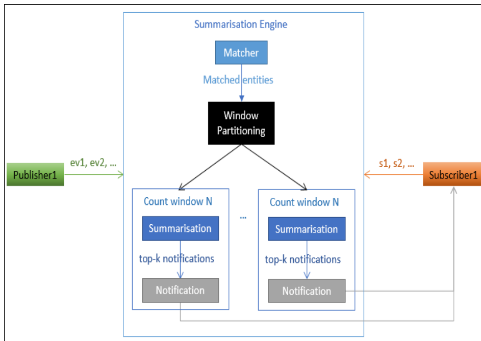
Figure 3. Entity summarisation architecture
