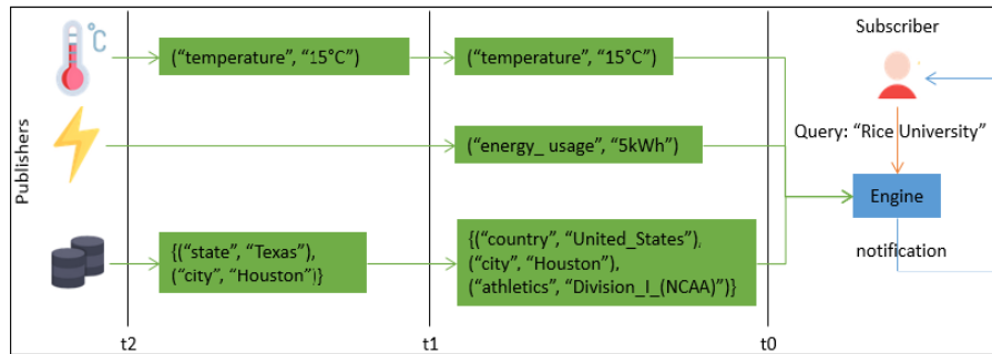
Figure 1. A subscriber is interested in information about Rice University and publishers publish timestamped information records about it. In this example, the temperature and city information is duplicate between timestamps t_2 and t_1
