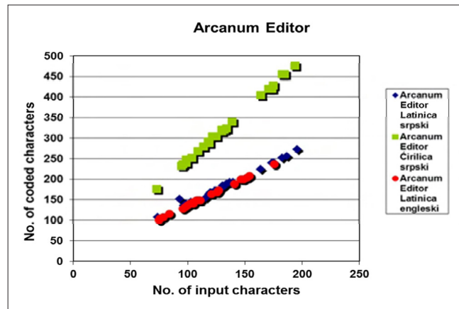
Figure 3. Coded vs. input text obtained by Arcanum Editor
