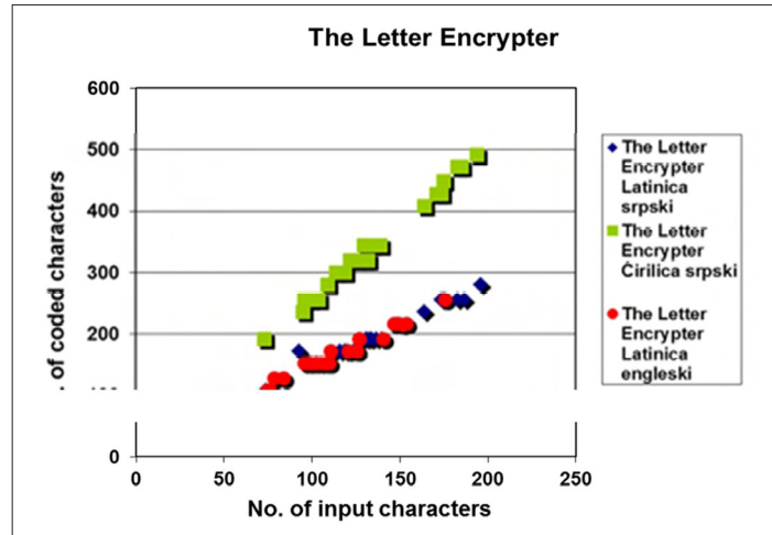
Figure 5. Coded vs. input text obtained by TheLetterEncrypter
