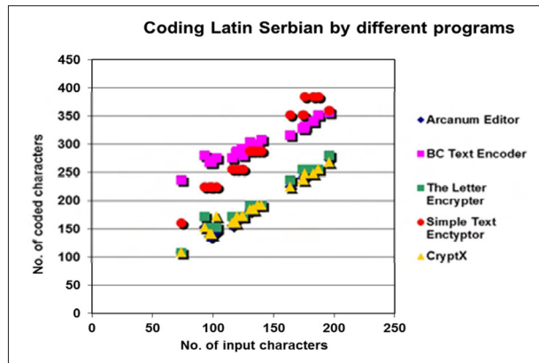
Figure 9. Coded vs. input Serbian Latin text
