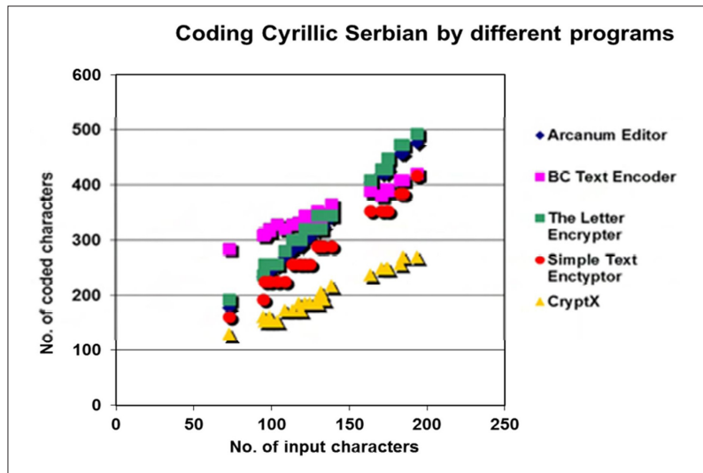
Figure 10. Coded vs. input Serbian Cyrillic text
