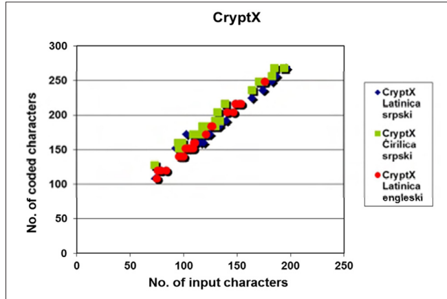
Figure 7. Coded vs. input text obtained by CryptX
