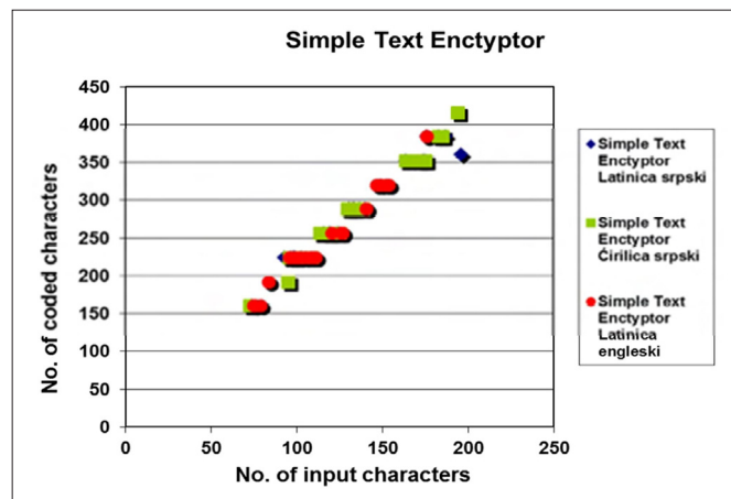
Figure 6. Coded vs. input text obtained by Simple Text Encryptor
