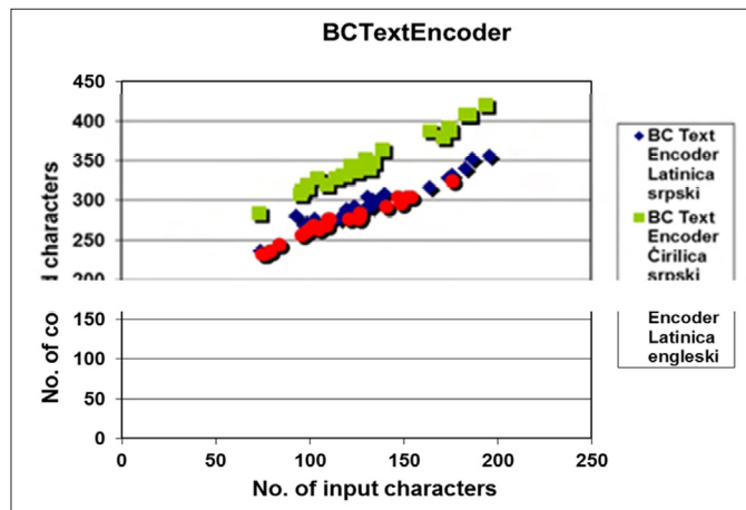
Figure 4. Coded vs. input text obtained by BCTextEncoder
