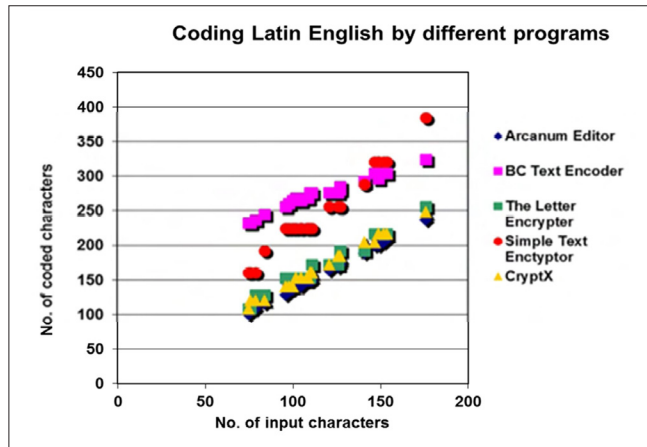
Figure 8. Coded vs. input English text
