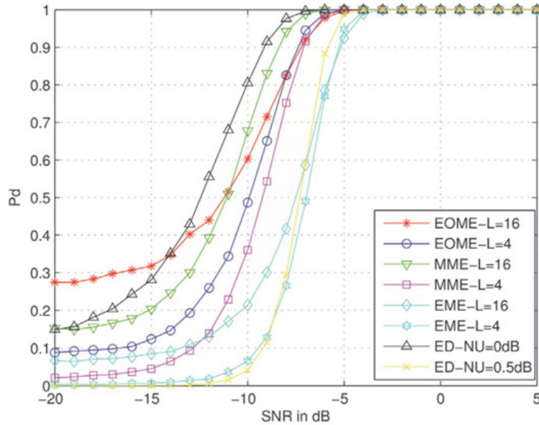
Figure 1. Simulation results for EOME, EME, MME, all with L = 4 and 16 and ED with 0 and 0.5 dB noise uncertainty sensing methods
