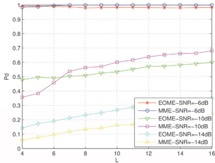
Figure 2. Simulation results for EOME and MME sensing methods with different smoothing factors in SNRs equal to -6 dB, -10 dB and -14 dB
