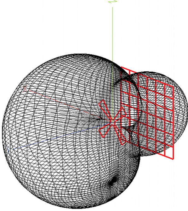
Figure 4. 3D radiation pattern of optimized X-pol antenna
