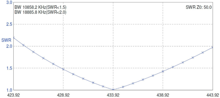
Figure 5. SWR behaviour in the working frequency range
