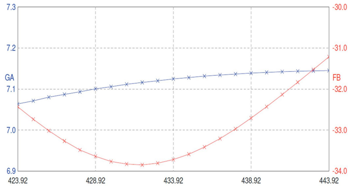
Figure 6. Gain and Front-to-back ratio behaviour in the working frequency range
