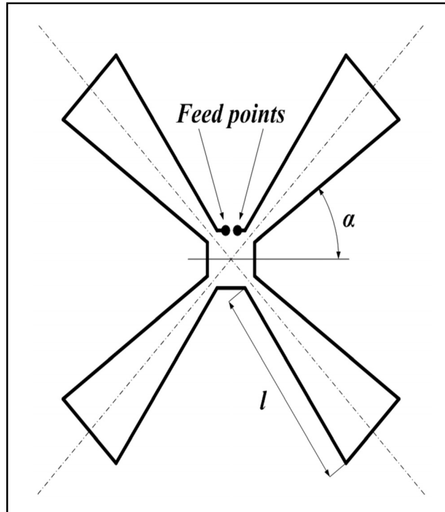
Figure 1. Structure of a planar radiating loop element of X-pol antenna
