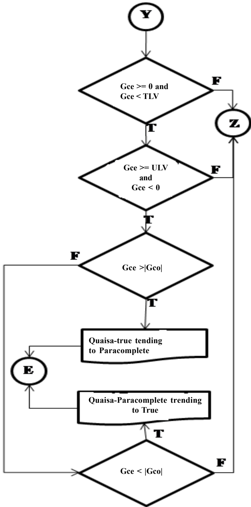
Figure 6. Paraconsistent logical flowchart: Quasi True tending to Paracompletenessn, Paracompletenessn tending to the True
