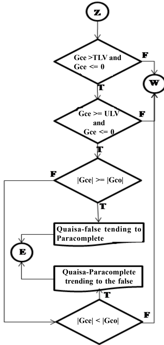
Figure 7. Paraconsistent logical flowchart: Quasi-False tending to Paracompletenessn, Paracompletenessn tending to False
