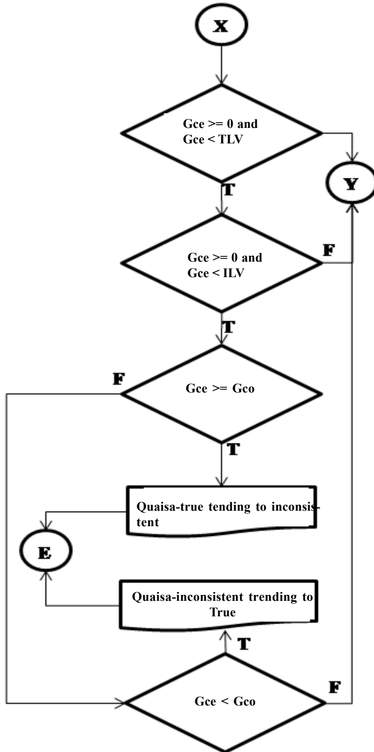
Figure 5. Paraconsistent logical flowchart: Quasi True tending to the Inconsistent, Inconsistent tending to True
