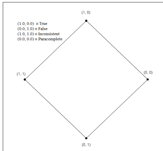
Figure 2. Paraconsistent Logical Lattice- Source: [11]
