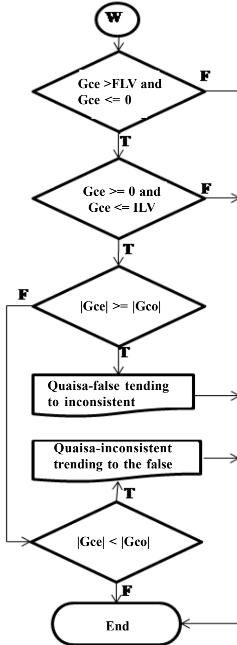
Figure 8. Paraconsistent logical flowchart: Quasi False tending to Inconsistent, Inconsistent tending to False (Source: Luiz A. de Lima).
