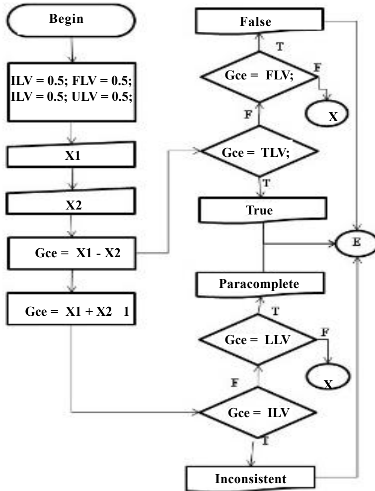
Figure 4. Paraconsistent logical flowchart: True, False, Inconsistent, Paracomplete
