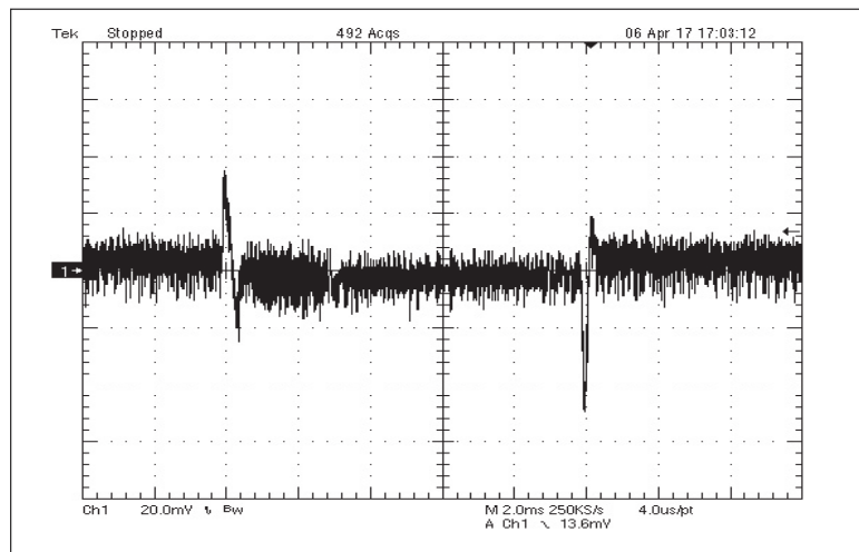
Figure 8. Output voltage load transient response
