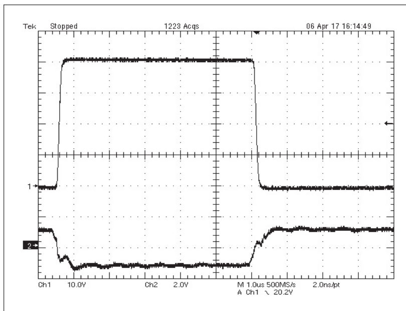
Figure 4. Drain and gate voltage of low side FET Q2 (zoomed in)
