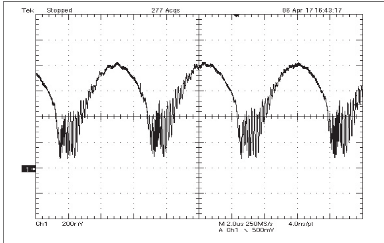
Figure 7. Primary current (rectified at current sense)
