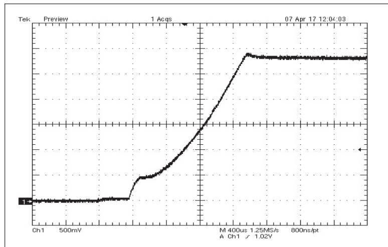
Figure 9. Output voltage rise into full load at turn on
