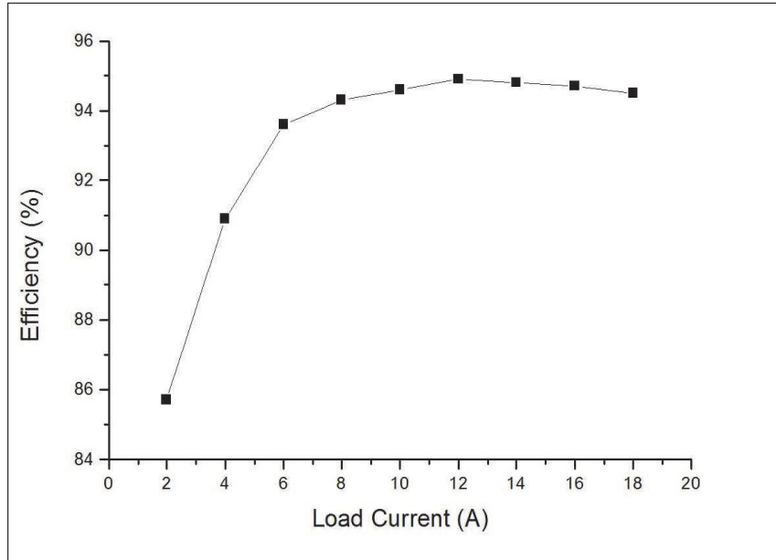
Figure 12. Efficiency vs. load current
