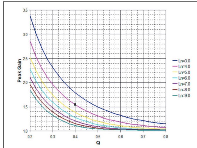
Figure 2. Peak gain curves
