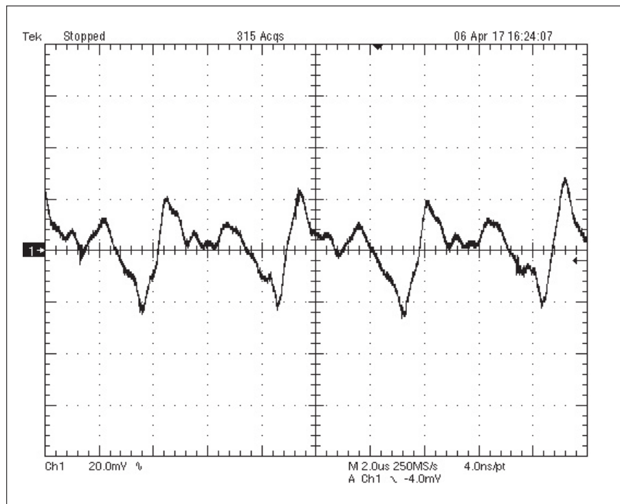
Figure 6. Output ripple at full load
