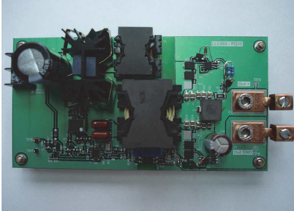
Figure 10. The converter prototype
