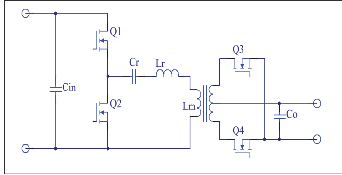
Figure 1. HB LLC converter
