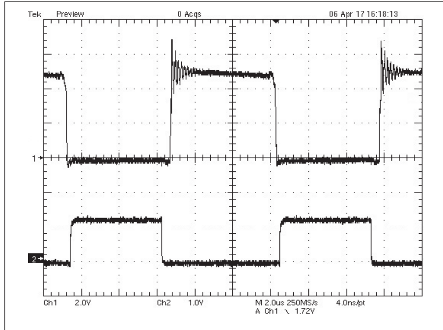
Figure 5. Drain and gate voltage of FET Q_4
