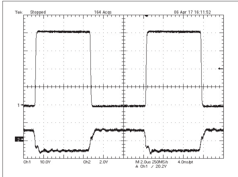
Figure 3. Drain and gate voltage of low side FET Q2
