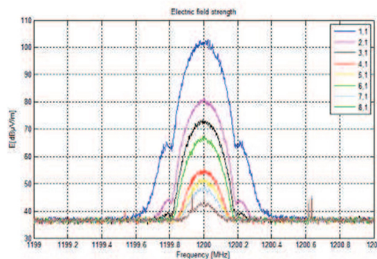
Figure 2. Series of Field Strength Curves on the Frequency 1200 Mhz for Different Distances from the Generator
