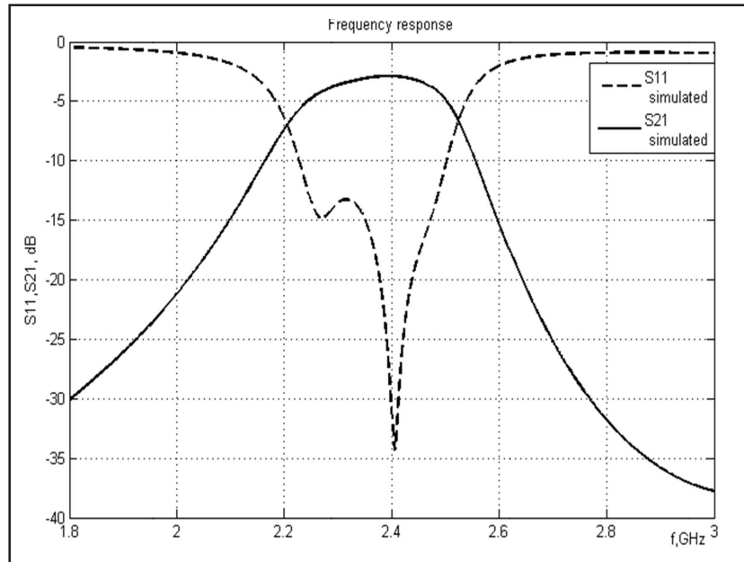
Figure 6. (b) Narrowband frequency response of the synthesized filter
