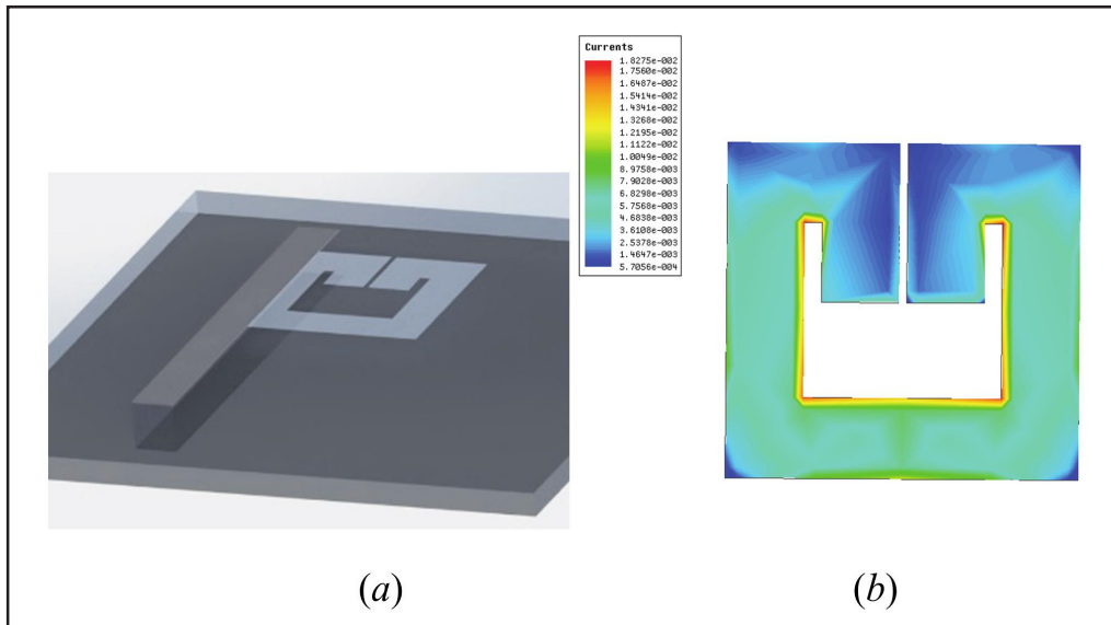
Figure 1. Topology (a) and electric field (b) distribution of miniaturized hairpin DGS resonator
