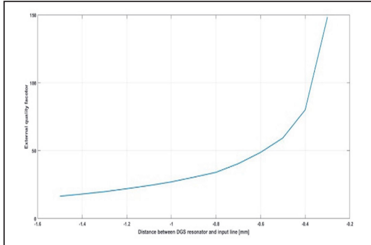
Figure 5. Dependence of the external coupling to the position of the input/output microstrip line
