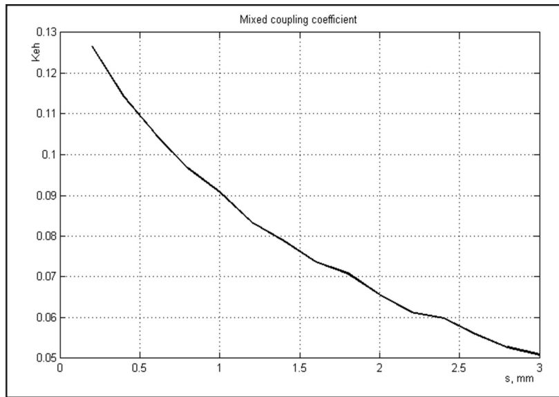
Figure 4 (c) Dependence of the coupling coefficient for mixed coupling
