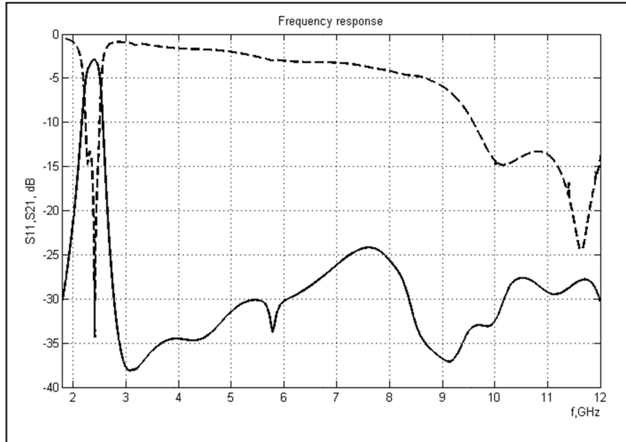
Figure 7. Wideband frequency response of the synthesized filter
