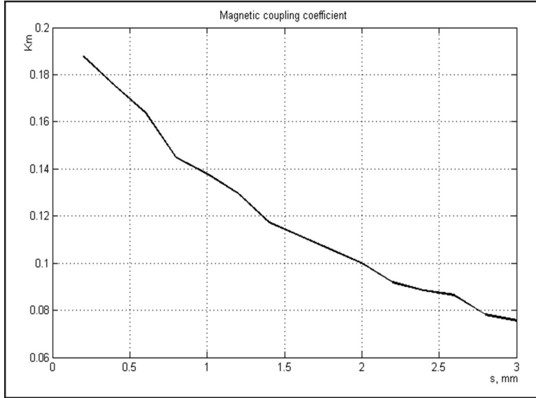
Figure 4. (b) Dependence of the coupling coefficient for magnetic coupling
