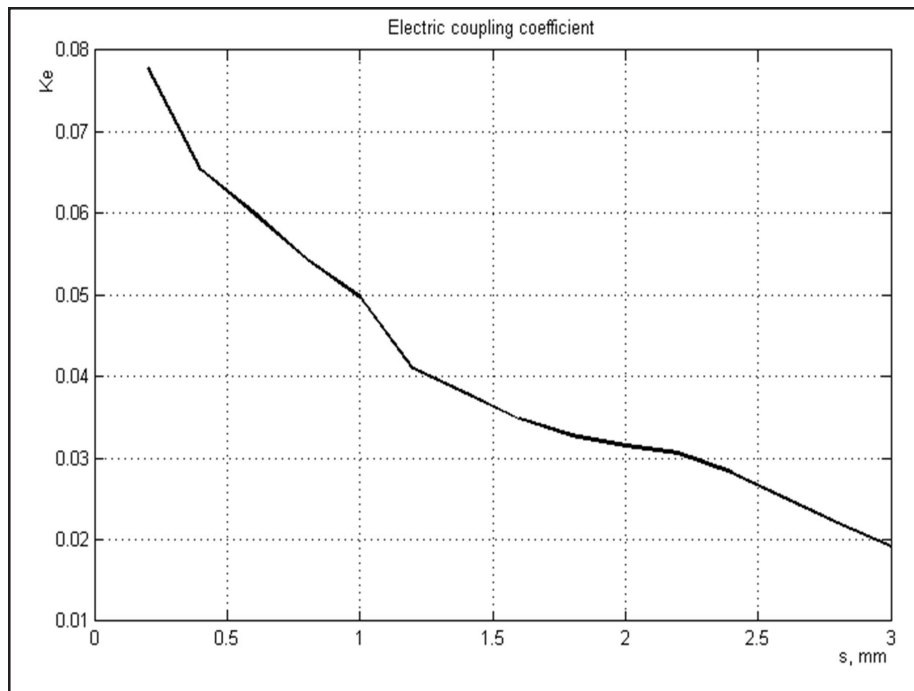
Figure 4. (a) Dependence of the coupling coefficient for electric coupling
