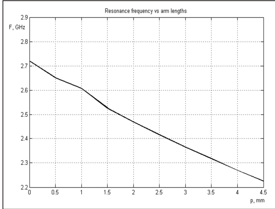
Figure 2. Dependence of the resonance frequency of the length of the coupled lines
