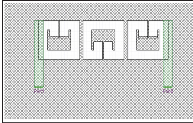
Figure 6. (a) Topology of the synthesized three resonator Chebyshev filter
