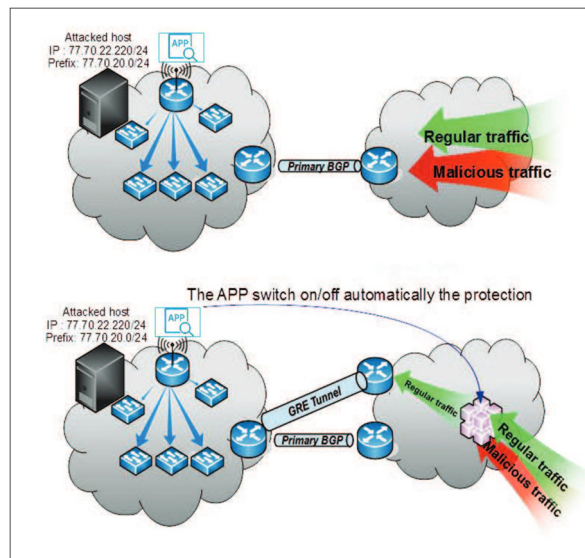
Figure 2. DDoS attack detection and notification
