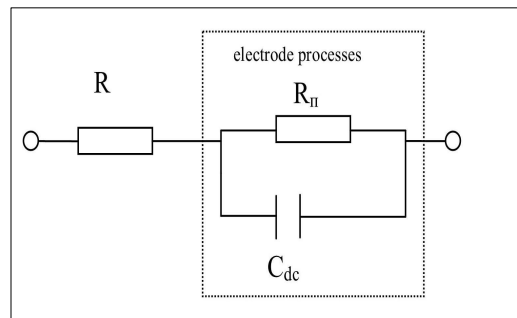
Figure 1. Randles model
