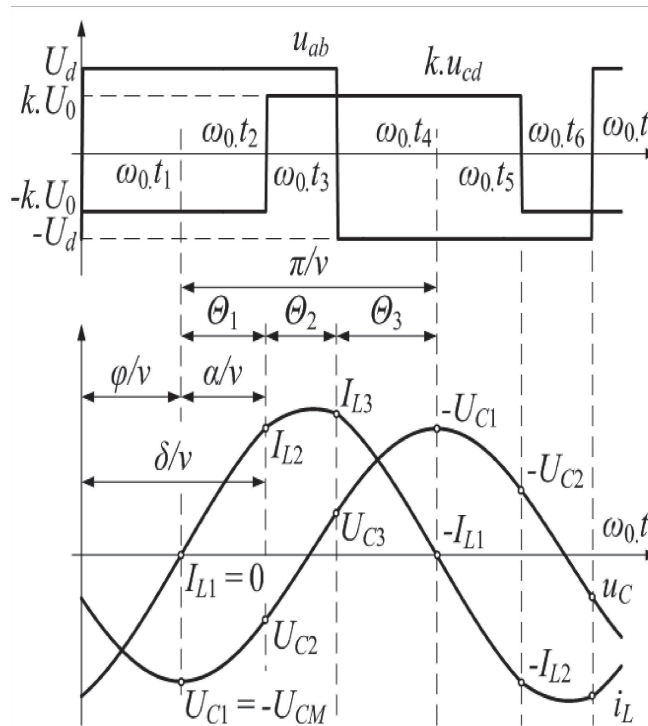
Figure 2. Waveforms at DIRECT MODE
