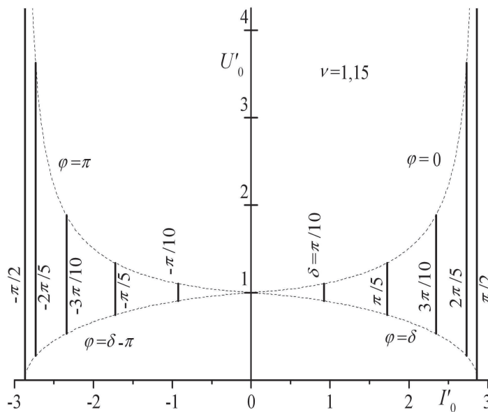
Figure 4. Normalized output characteristics at -\pi/2 \leq \delta \leq +\pi/2
