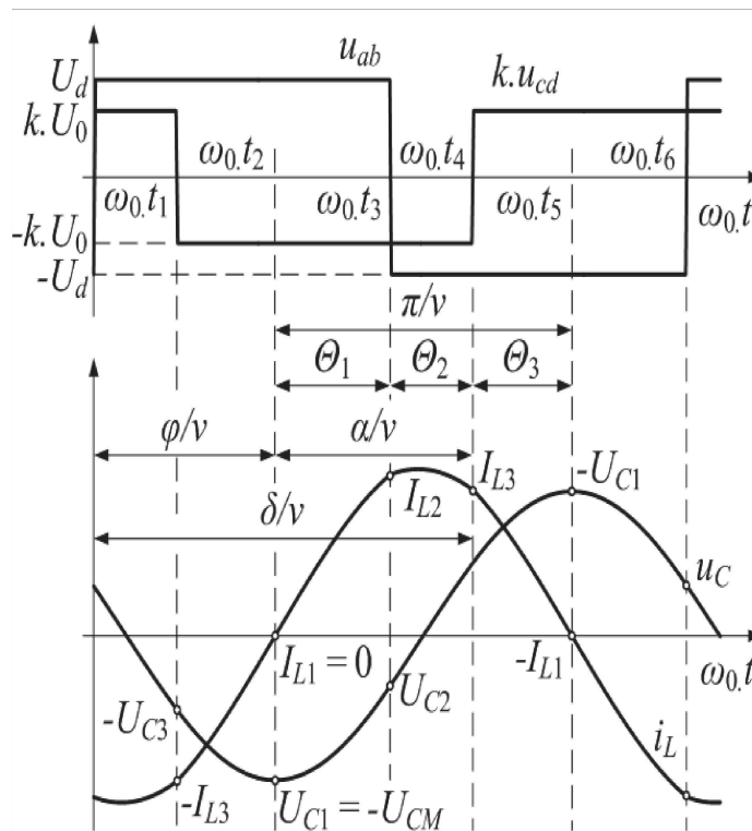
Figure 2. Waveforms at DIRECT MODE
