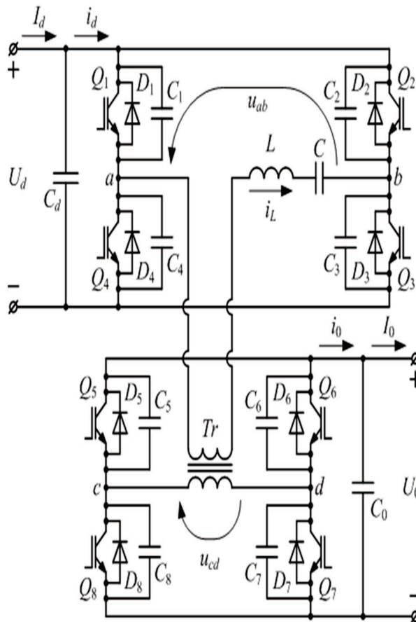
Figure 1. Circuit of the Bidirectional Resonant DC/DC Converter
