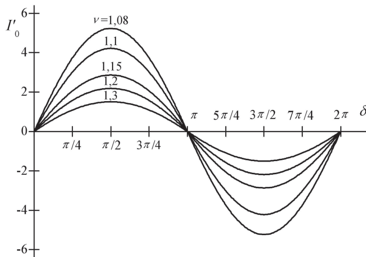
Figure 8. Normalized control characteristics of the converter
