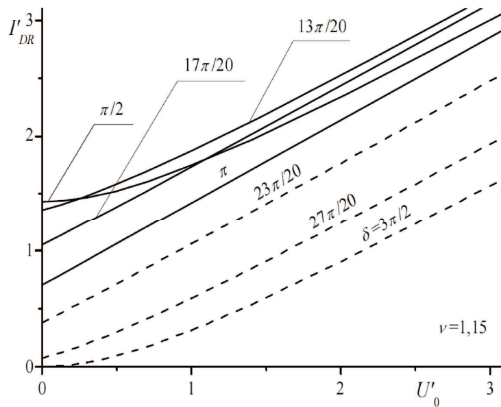
Figure 7. Normalized average current through the “output” stage freewheeling diodes – I'_{DR}
