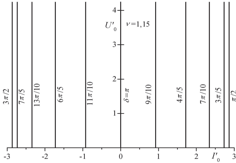
Figure 5. Normalized output characteristics at \pi/2 \leq \delta \leq 3\pi/2
