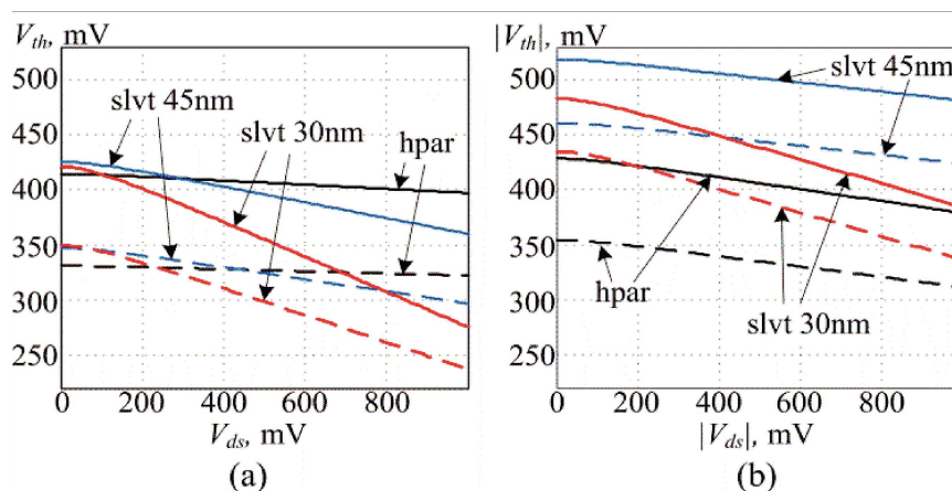
Figure 3. Dependence of the threshold voltage from the drain-source voltage for the transistors of interest. Solid lines - with bulk effect, dashed lines - without bulk effects: (a) NMOS; (b) PMOS
