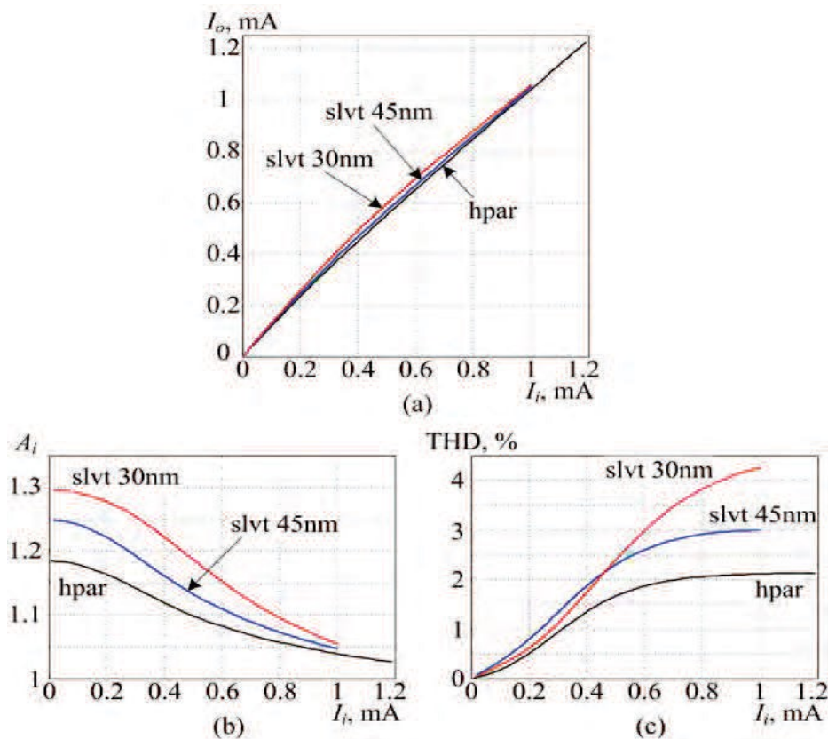
Figure 6. Dependences of large signal parameters of the designed amplifiers from the input current: (a) output current; (b) large signal current gain; (c) THD
