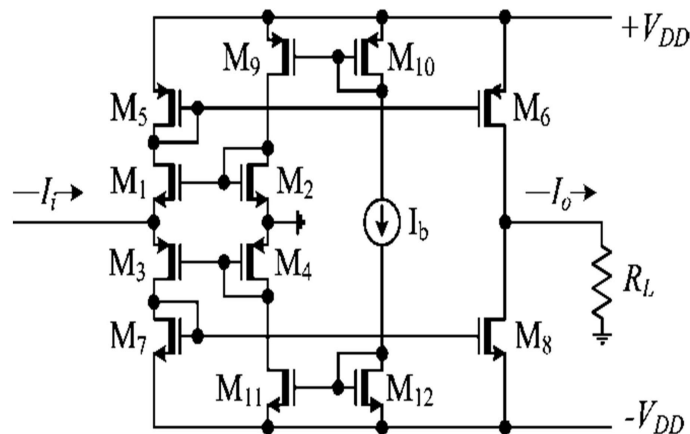
Figure 1. The circuit of the current amplifier
