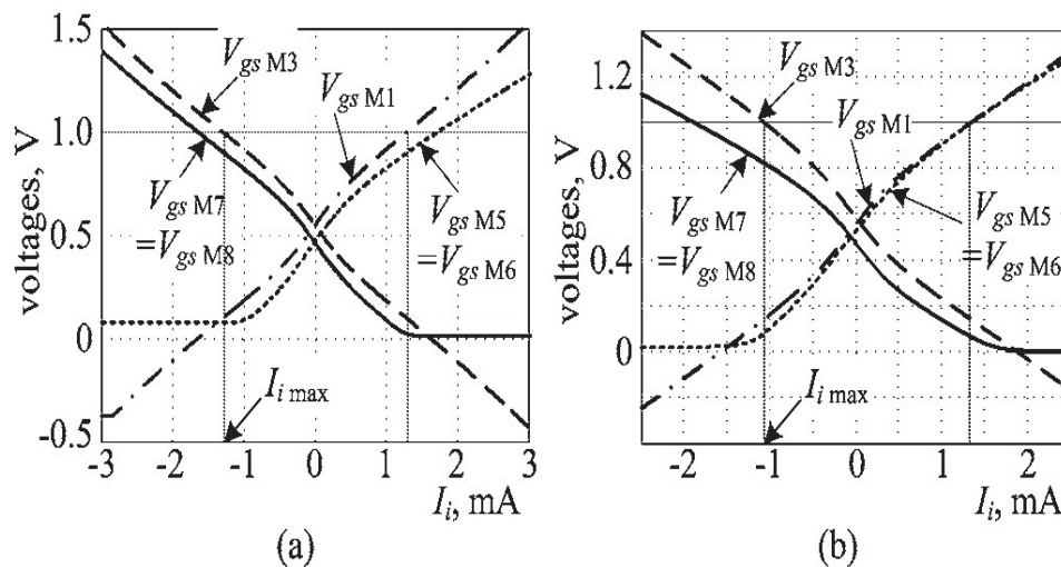
Figure 4. Gate-source voltages, which exceed the safe operation range: (a) amplifier with hpar FETs, (b) amplifier with slvt 45nm FETs
