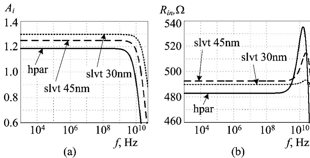
Figure 5. Small signal characteristics of the designed amplifiers: (a) current gain; (b) input impedance
