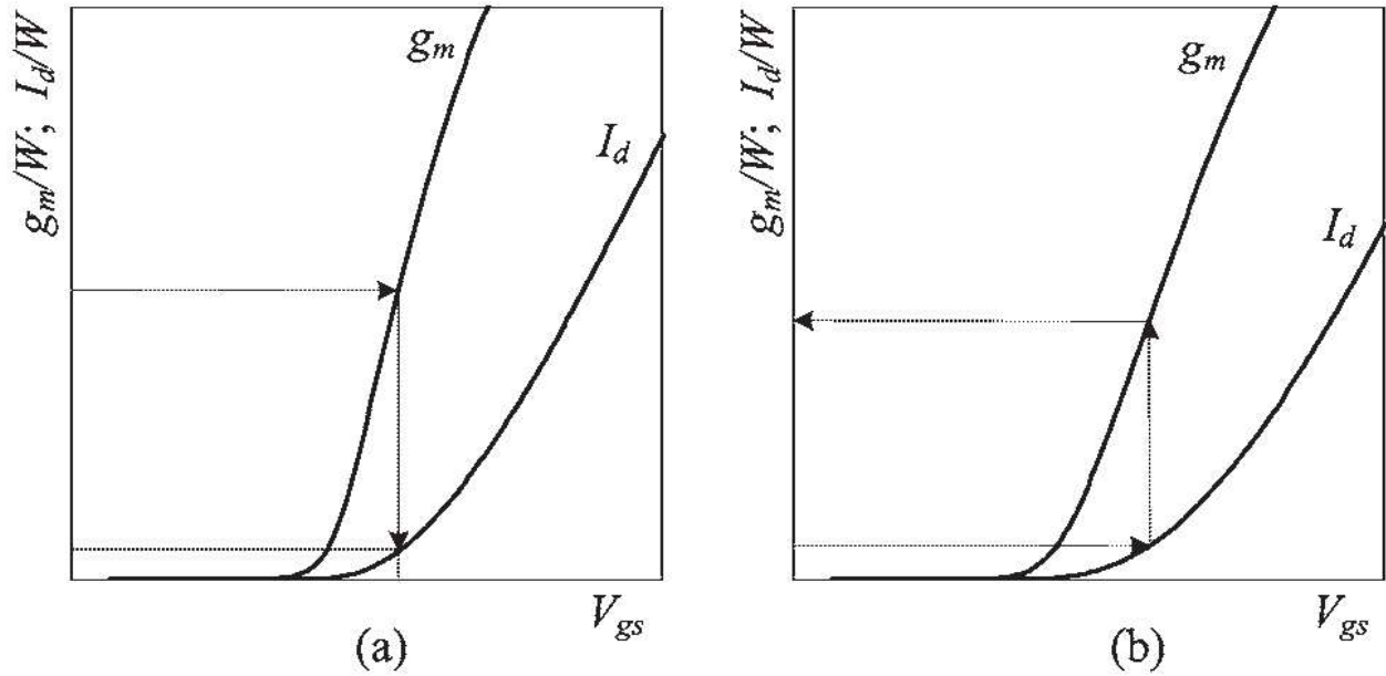
Figure 2. Plots of normalized g_m and ID vs. V_{GS} : (a) NMOS; (b) PMOS
