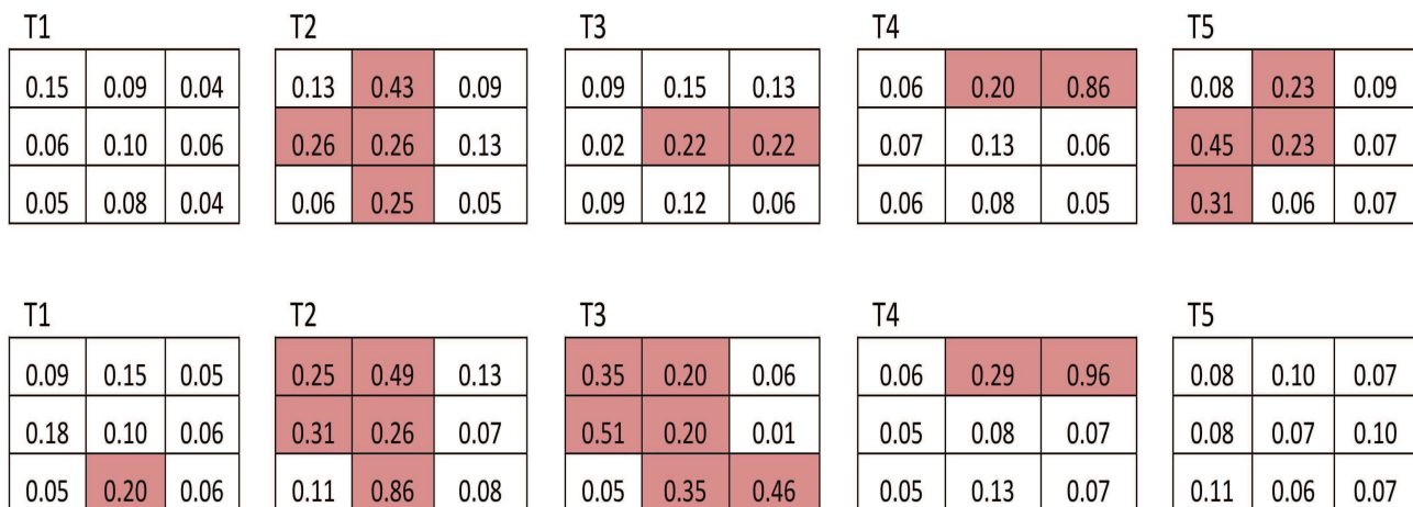
Figure 3. Magnetic field measurement level (Top position represents measurement at the top of the tablet (touchscreen display area). Bottom position represents measurement at the bottom areas of the tablet. Colored fields represent the areas with higher emission than it is allowed)
