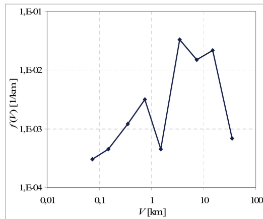
Figure 1. Probability density function f(V) of meteorological distance of visibility V
