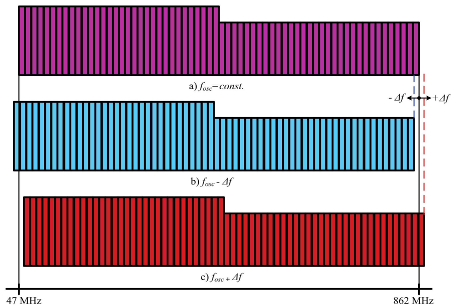
Figure 3. CATV/HFC system's spectrum
