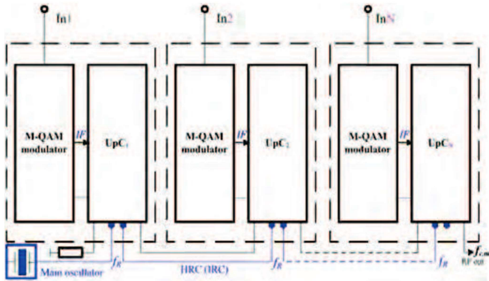
Figure 2. Structural schematic of Head End with coherent carriers
