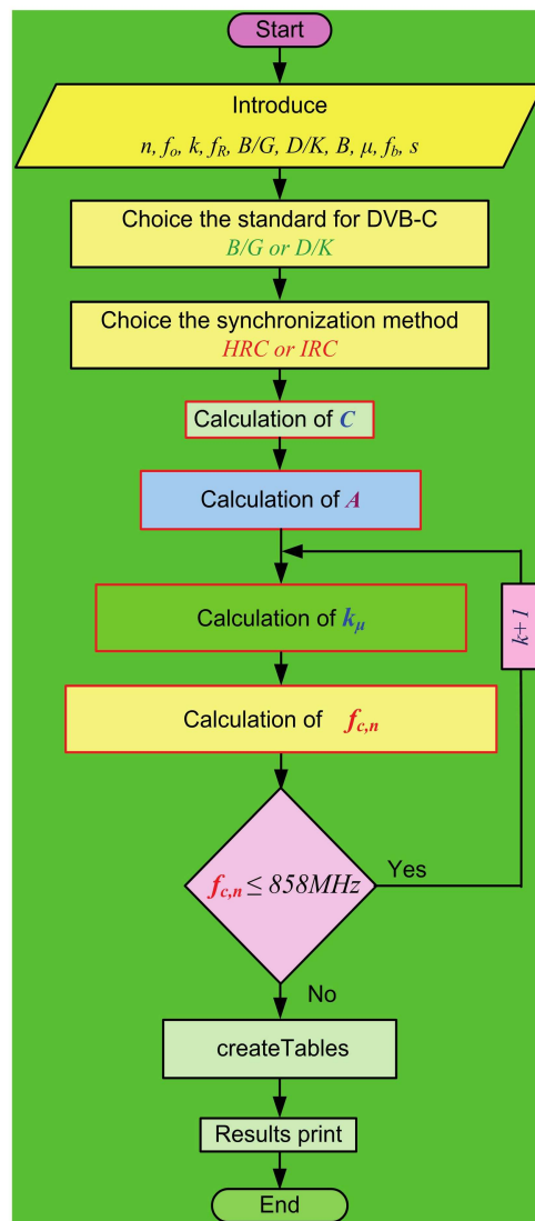
Figure 4. Algorithm for calculating the digital carrier
