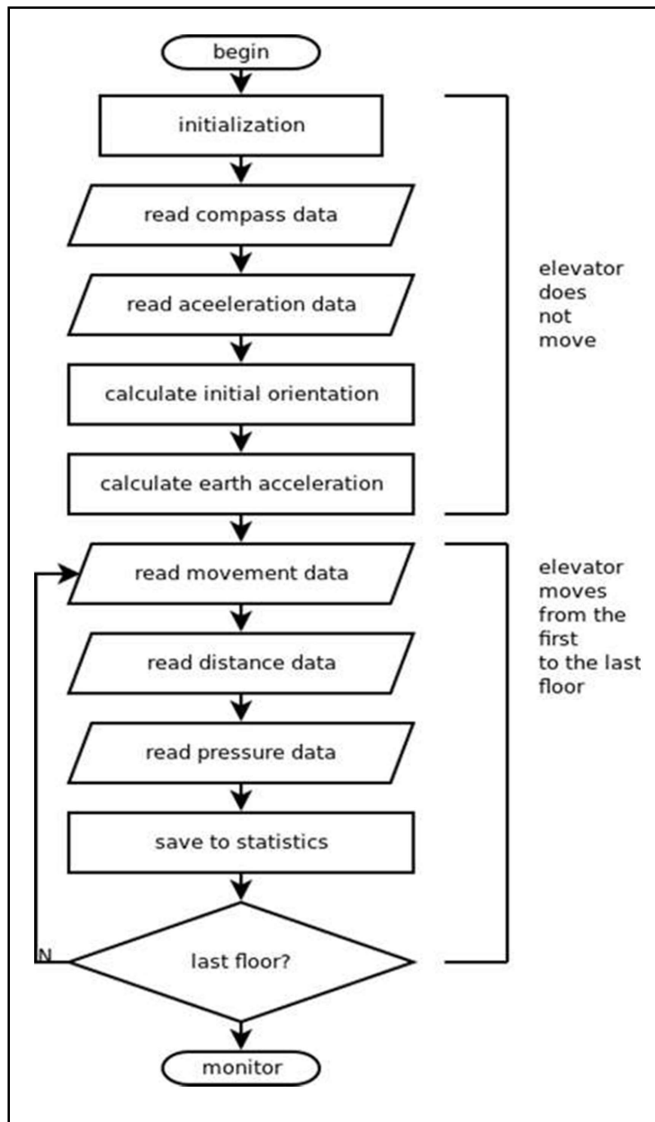
Figure 2. Software diagram for initial data calibration
