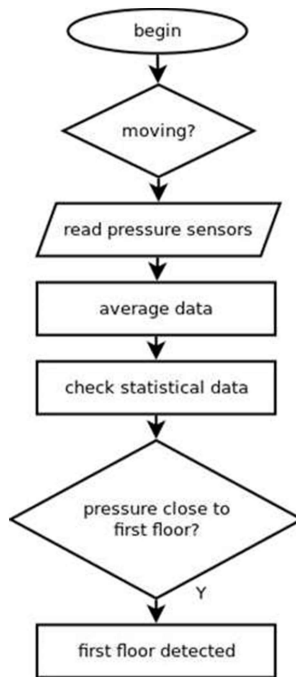
Figure 3. Software diagram for detecting first floor
