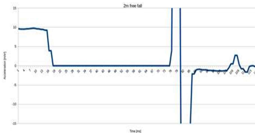
Figure 4. Free fall data accelerometer MPU6050. X axis time; Y axis acceleration m/s 2
