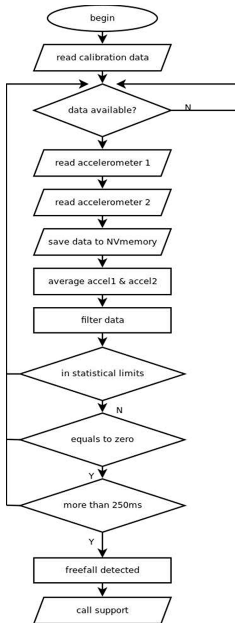
Figure 5. Free fall data accelerometer MPU6050
