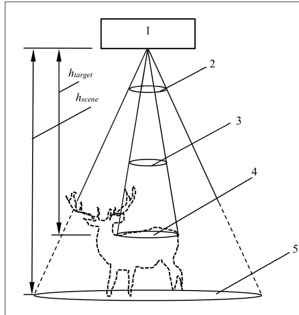
Figure 1. General set-up of a wild animal radiometric investigation (1- radiometric device; 2-solid view angle of the radiometric device; 3- solid view angle of the animal investigated; 4-essential area of the wild animal surface which produces radiation (target); 5-radiation from the surface on which the animal is located (scene), h_{target} - distance to the target, h_{scene} distance to the scene)
