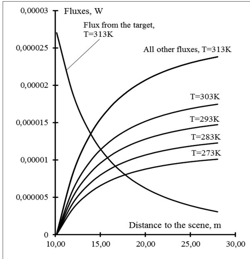
Figure 2. Simulation for one type of target with temperature 313K and emissivity coefficient 0,99 (wild animal) and different temperatures for a scene with emissivity coefficient 0,98 and atmosphere
