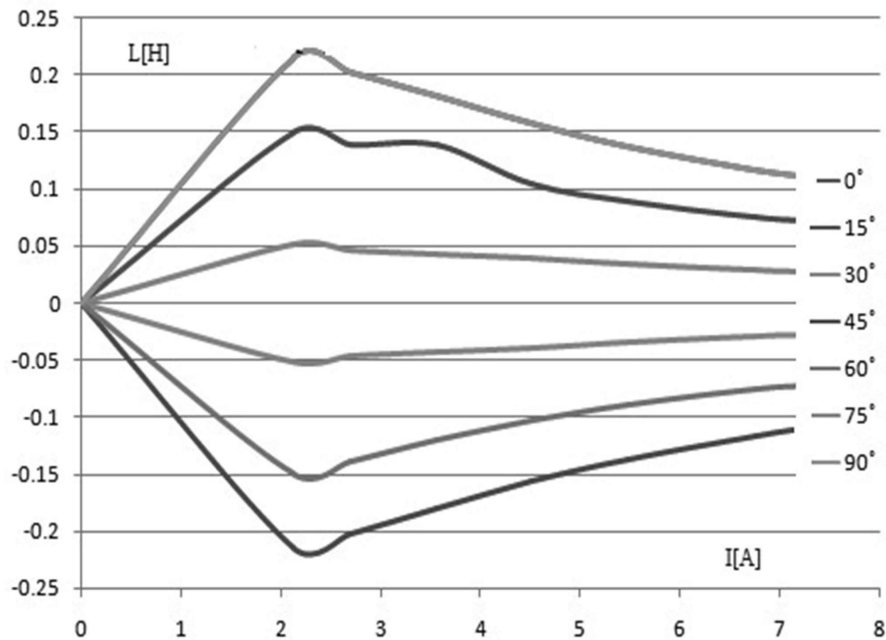
Figure 2. Equivalent inductance of the induction motor with double cage for various load currents and constant position of the rotor relative to the stator magnetic axis
