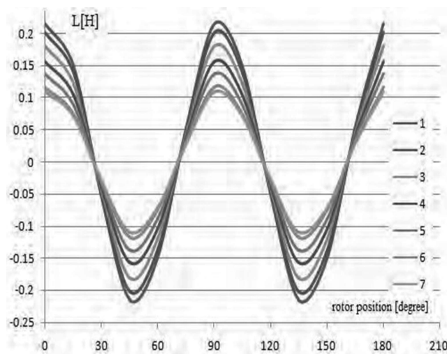
Figure 1. Equivalent inductance of air gap of induction motor with double cage at different angular positions of the rotor relative to the stator magnetic axis
