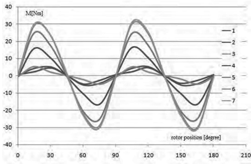
Figure 3. Characteristics of the electromagnetic torque
