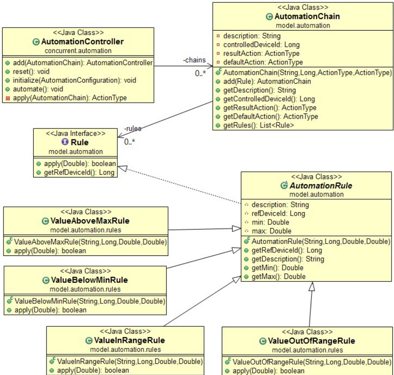
Figure 4. Model of automatic control of RAU
