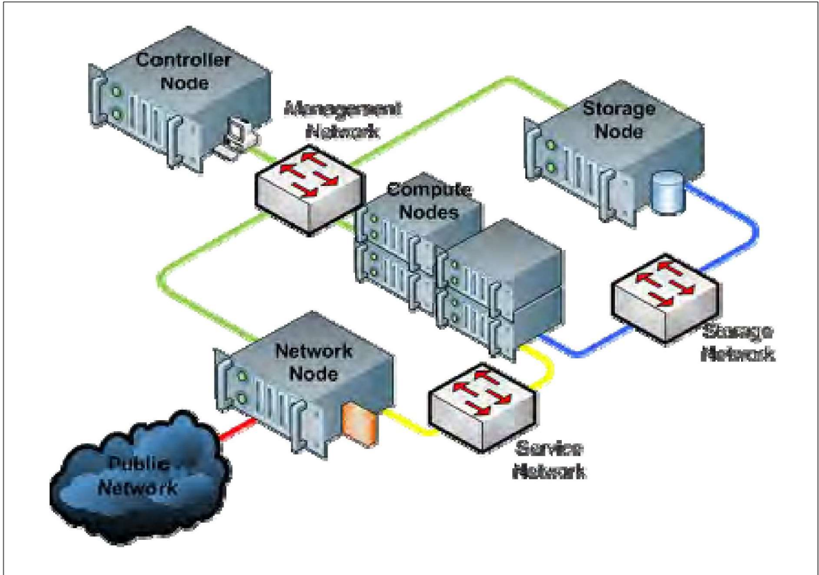
Figure 1. Architecture of the OpenStack Cloud Platform [18]
