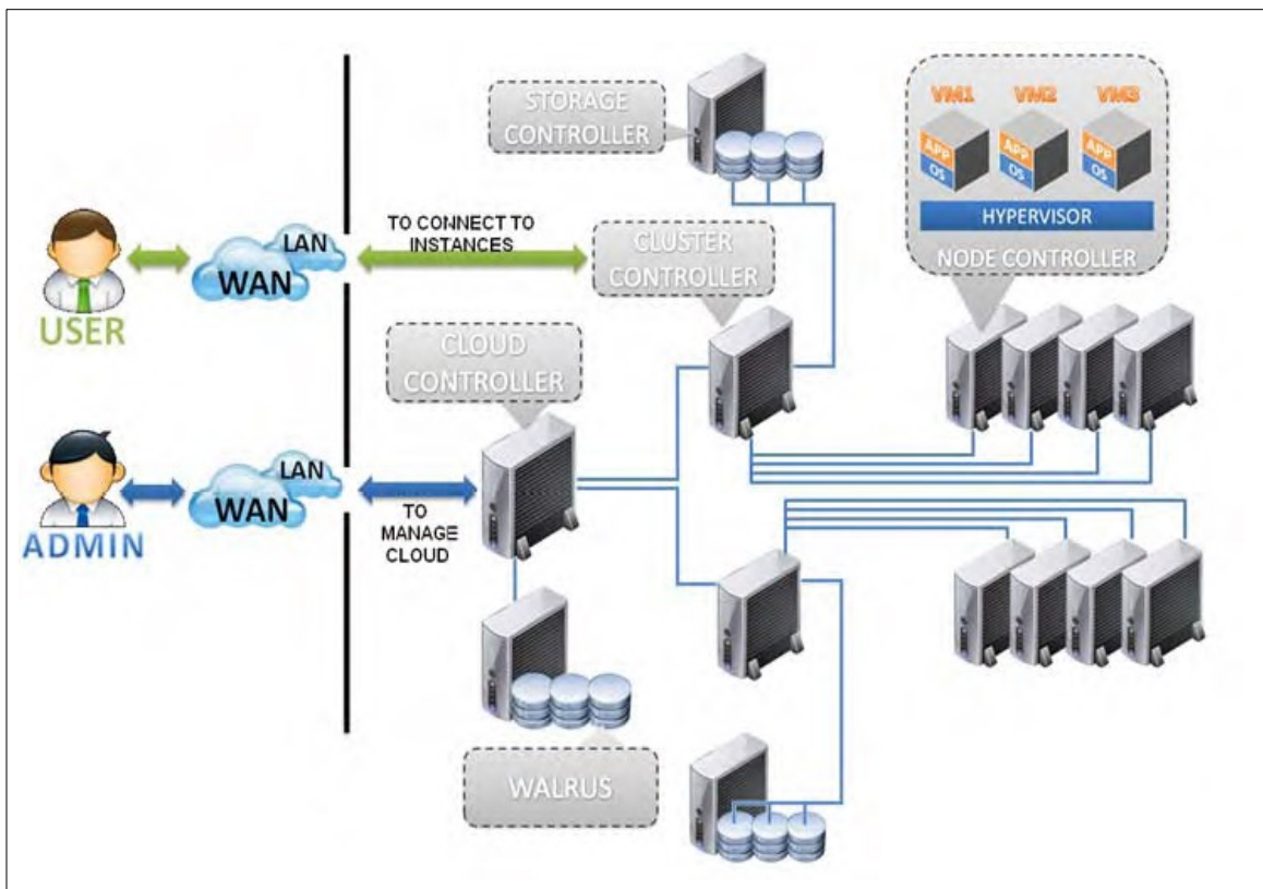
Figure 2. Architecture of the Eucalyptus Cloud Platform [19]
