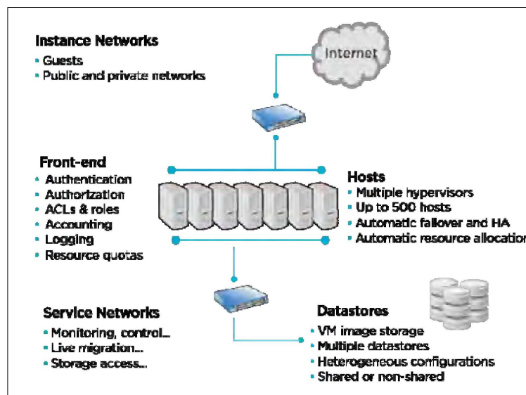
Figure 3. Architecture of the OpenNebula Cloud Platform [20]
