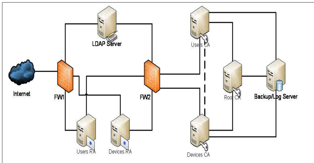
Figure 2. Architecture of INDECT PKI [6]
