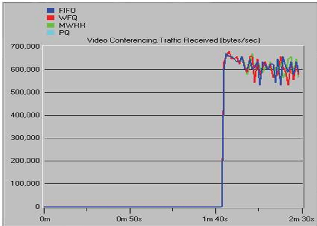
Figure 4. Video-conferencing traffic received (bytes/sec)
