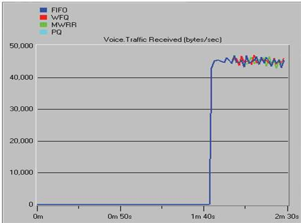
Figure 5. Voice traffic received (bytes/sec)
