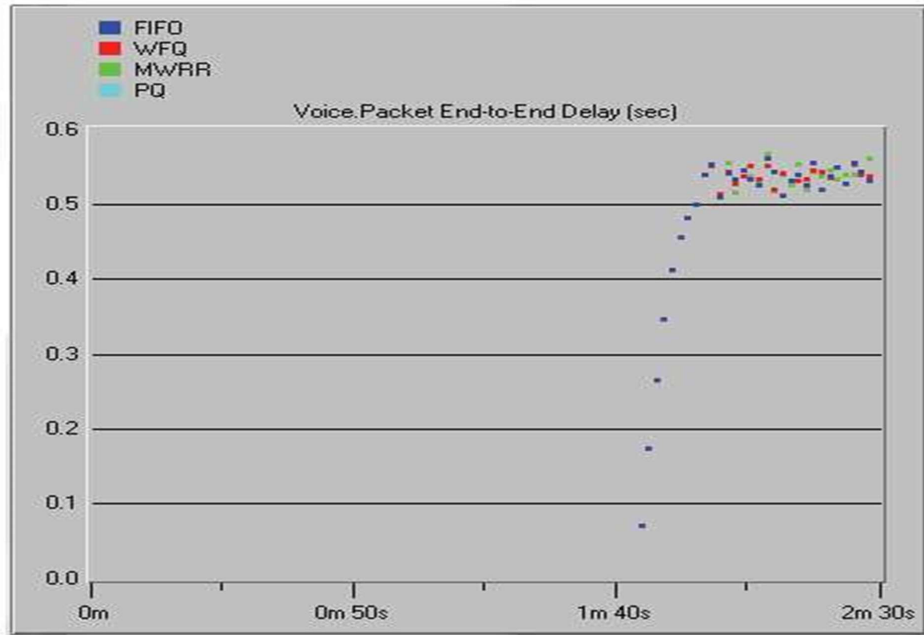
Figure 6. Voice packet end-to-end (sec)
