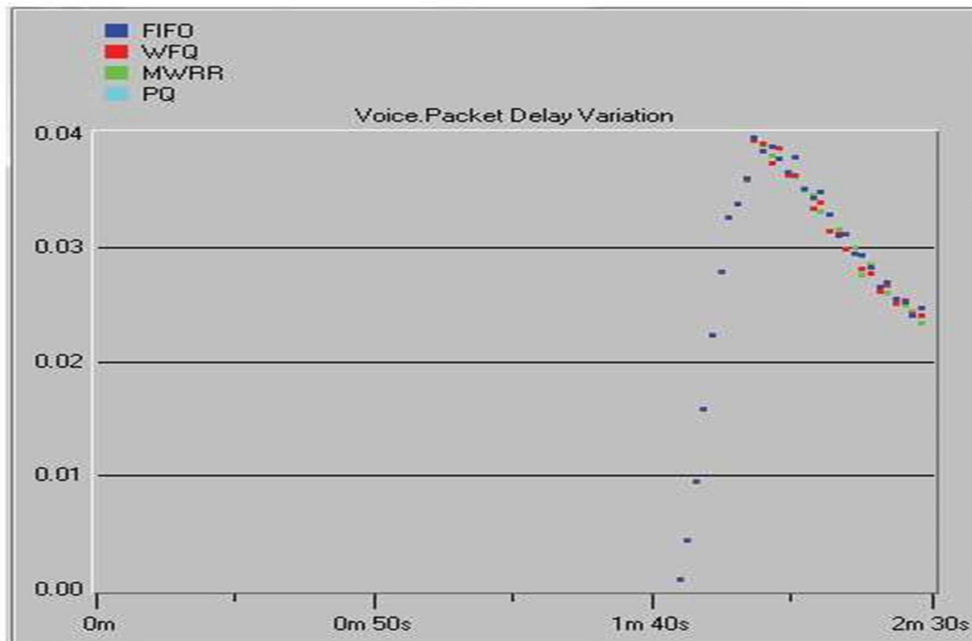
Figure 7. Voice packet delay variation (sec)
