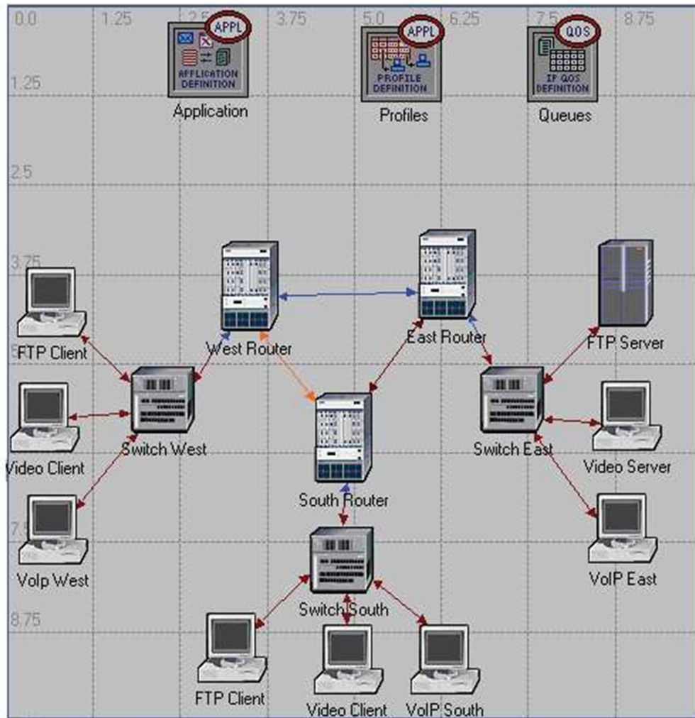
Figure 1. The network topology of the model
