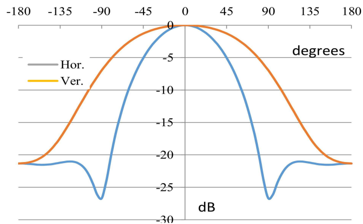
Figure 8. Radiation pattern for 1800 MHz
