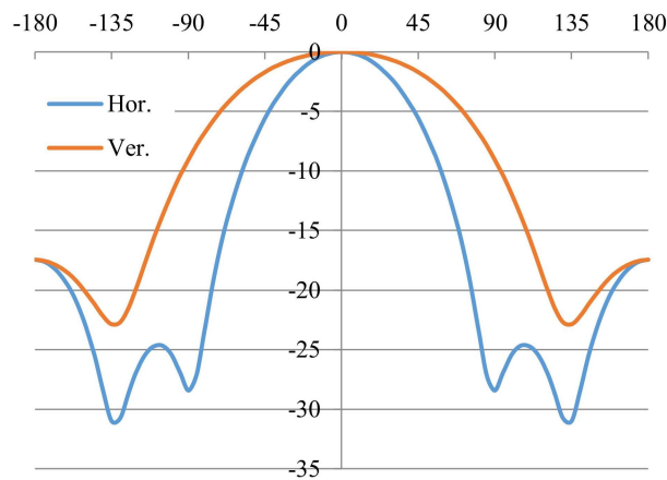
Figure 9. Radiation pattern for 1880 MHz
