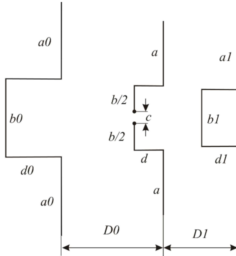
Figure 3. Proposed antenna design
