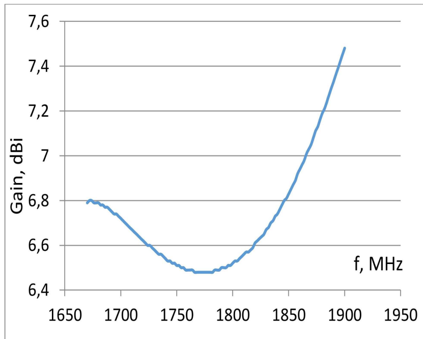
Figure 5. Antenna Gain
