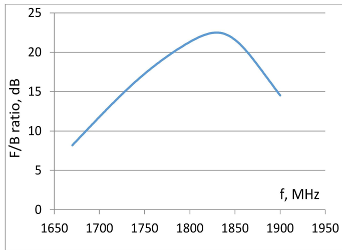
Figure 6. Front-to-back ratio
