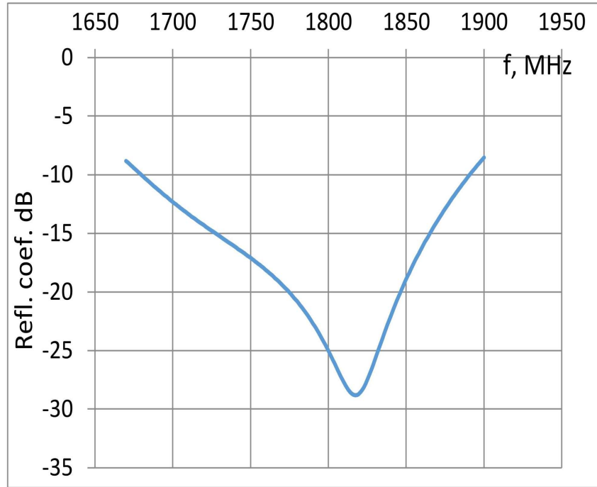
Figure 4. Return losses
