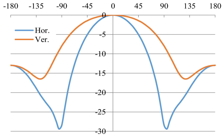
Figure 7. Radiation pattern for 1710 MHz
