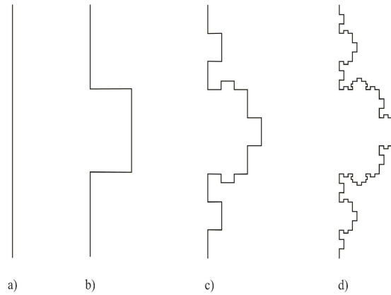
Figure 1. Minkowski curve: a) initiator; b) first iteration; c) second iteration d) third iteration
