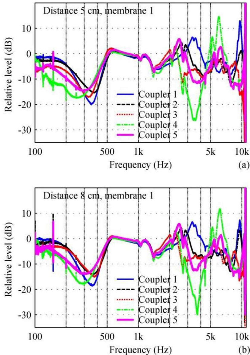
Figure 9. Differences between transfer functions measured with particular coupler with membrane 1 and without the membrane for microphone distance of (a) 5 cm and (b) 8 cm
