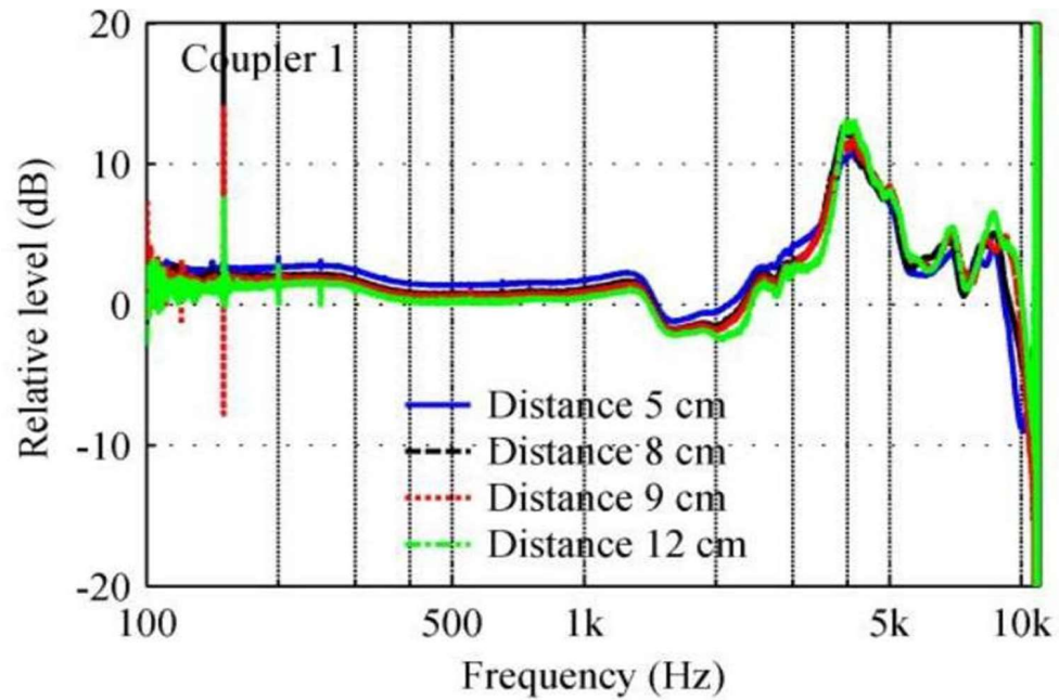
Figure 7. Transfer functions of the coupler 1 obtained as a difference of the transfer functions measured with and without coupler for different microphone distances
