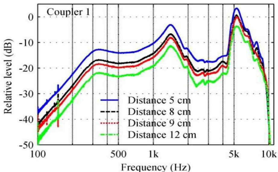
Figure 6. Transfer functions measured with coupler 1 and without speech membrane for different microphone distances
