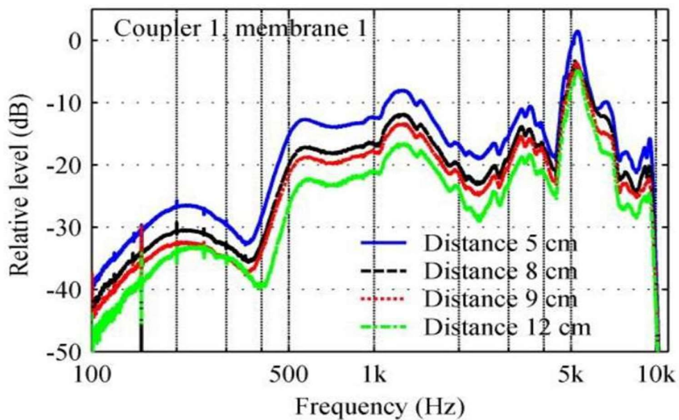
Figure 8. Transfer functions measured with coupler 1 and membrane 1 for different microphone distances
