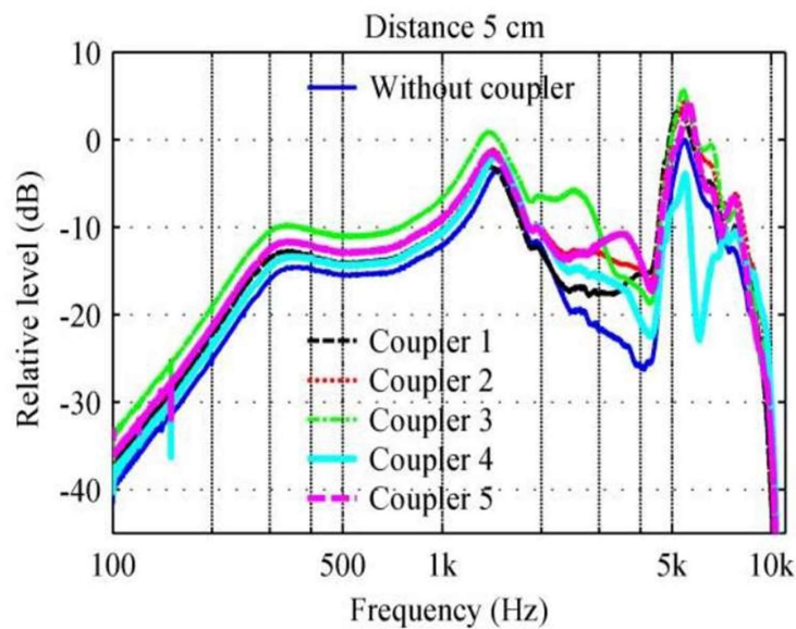
Figure 5. Transfer functions measured without coupler and with all 5 couplers without membrane for microphone distance of 5 cm
