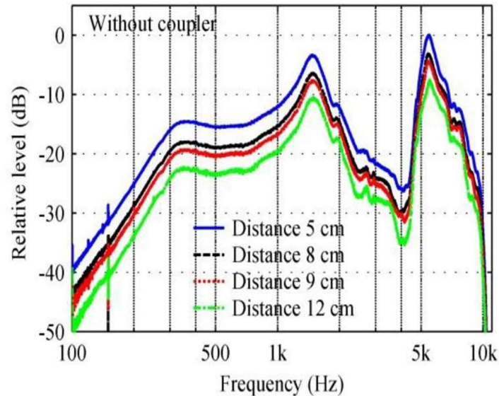
Figure 4. Transfer functions of the artificial mouth without coupler and membrane measured at different microphone distances
