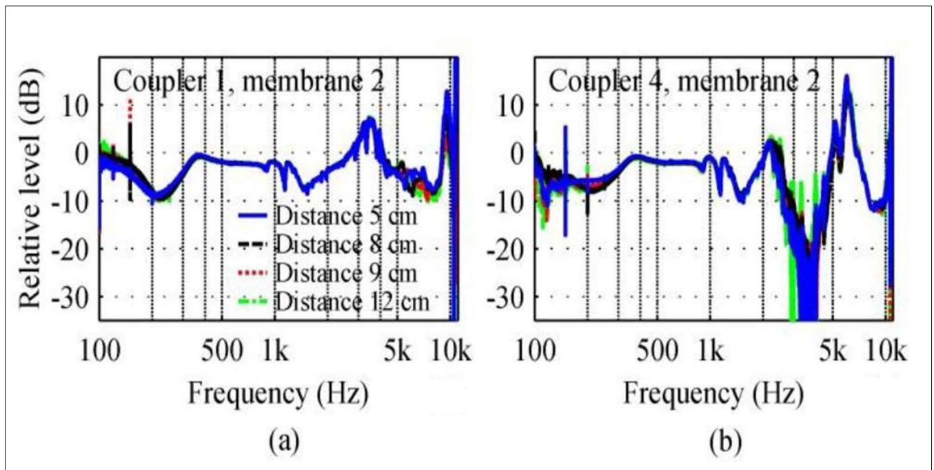
Figure 11. Differences between transfer functions measured with coupler (a) 1 and (b) coupler 4 with membrane 2 and without the membrane for different microphone distances
