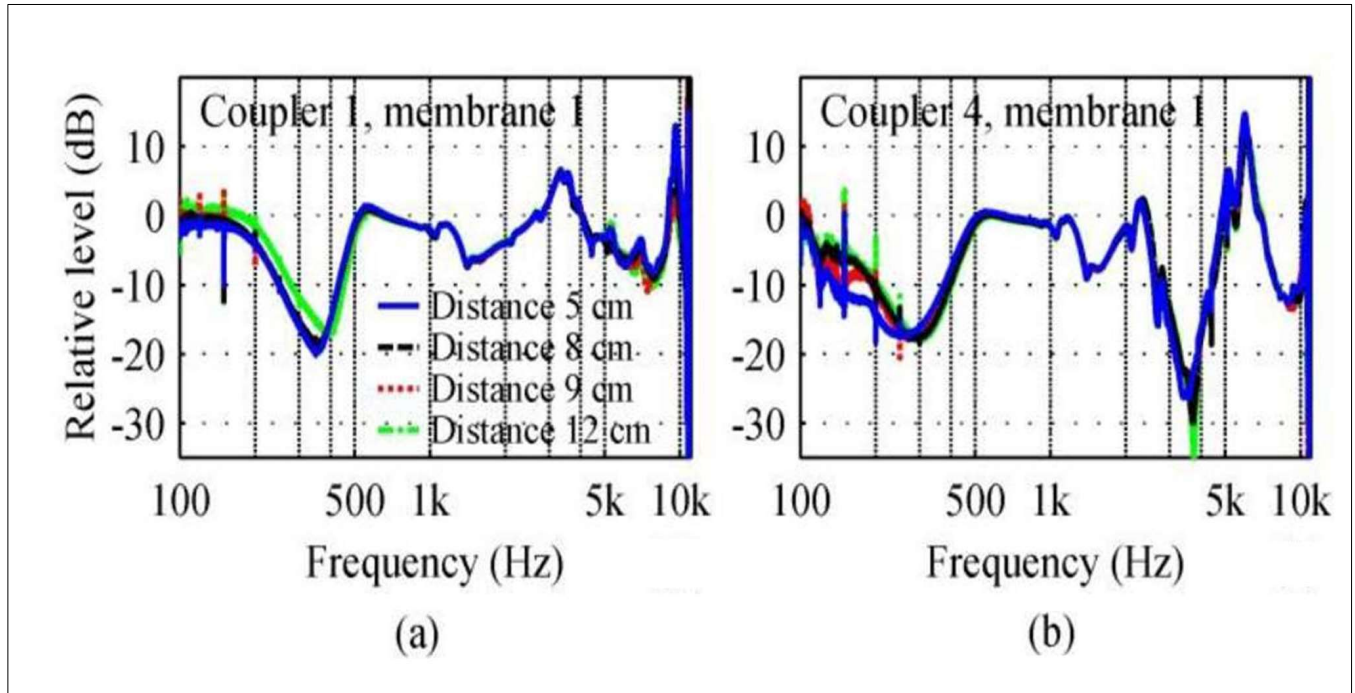
Figure 10. Differences between transfer functions measured with coupler (a) 1 and (b) coupler 4 with membrane 1 and without the membrane for different microphone distances
