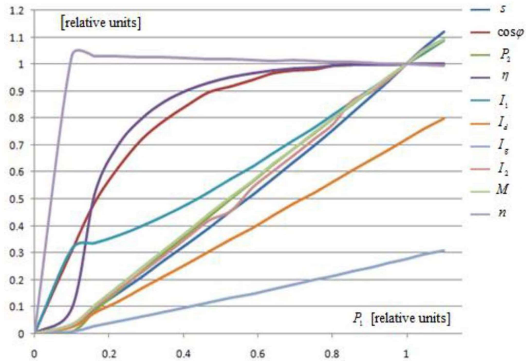
Figure 2. Operating characteristics of an asynchronous motor with a double cage
