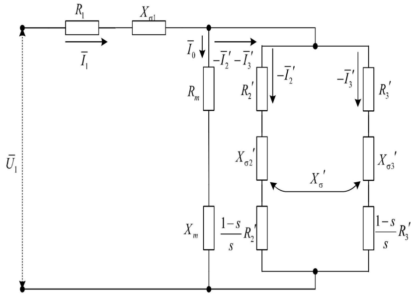
Figure 1. Asynchronous motor with double cage - equivalent electric scheme
