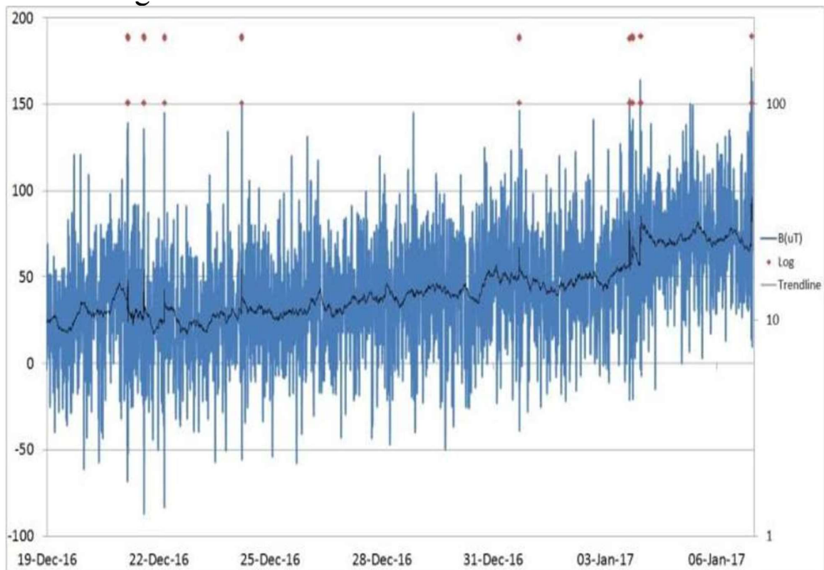
Figure 5. Magnetic field data
