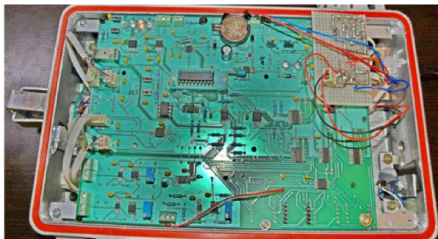
Figure 1. Evaluation board of the Adaptive Weather Station
