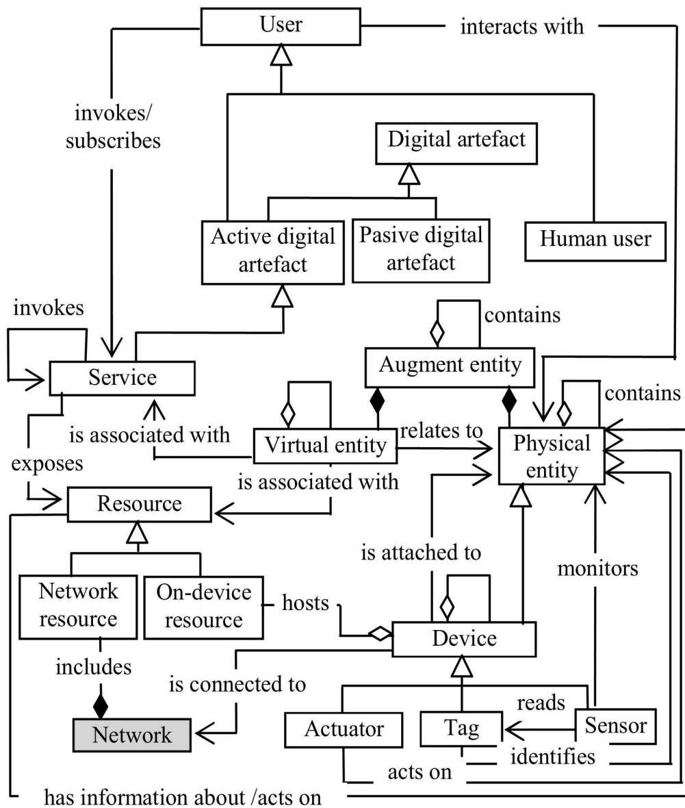
Figure 1. IoT Domain model [16] (the suggested enhancement is shown in grey)
