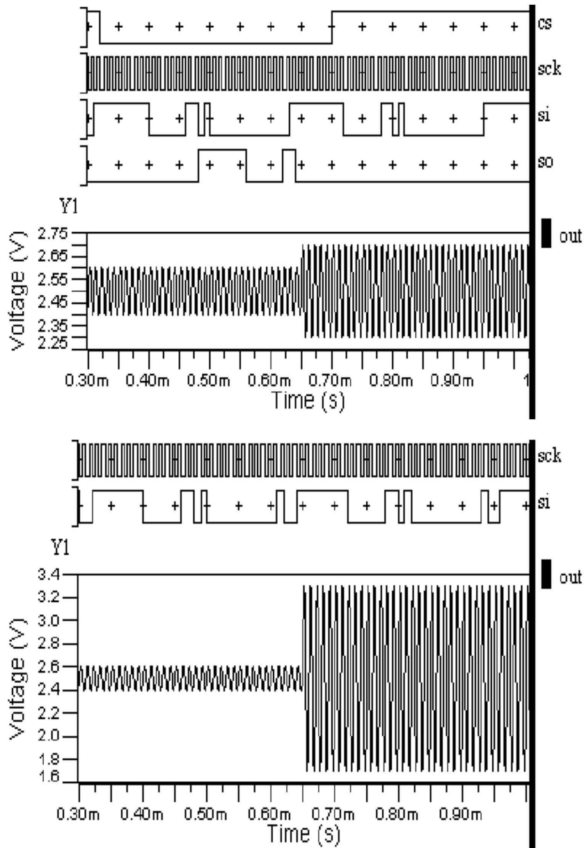
Figure 4. The simulated time domain responses for the proposed PGA model at gain 2 and 8, respectively
