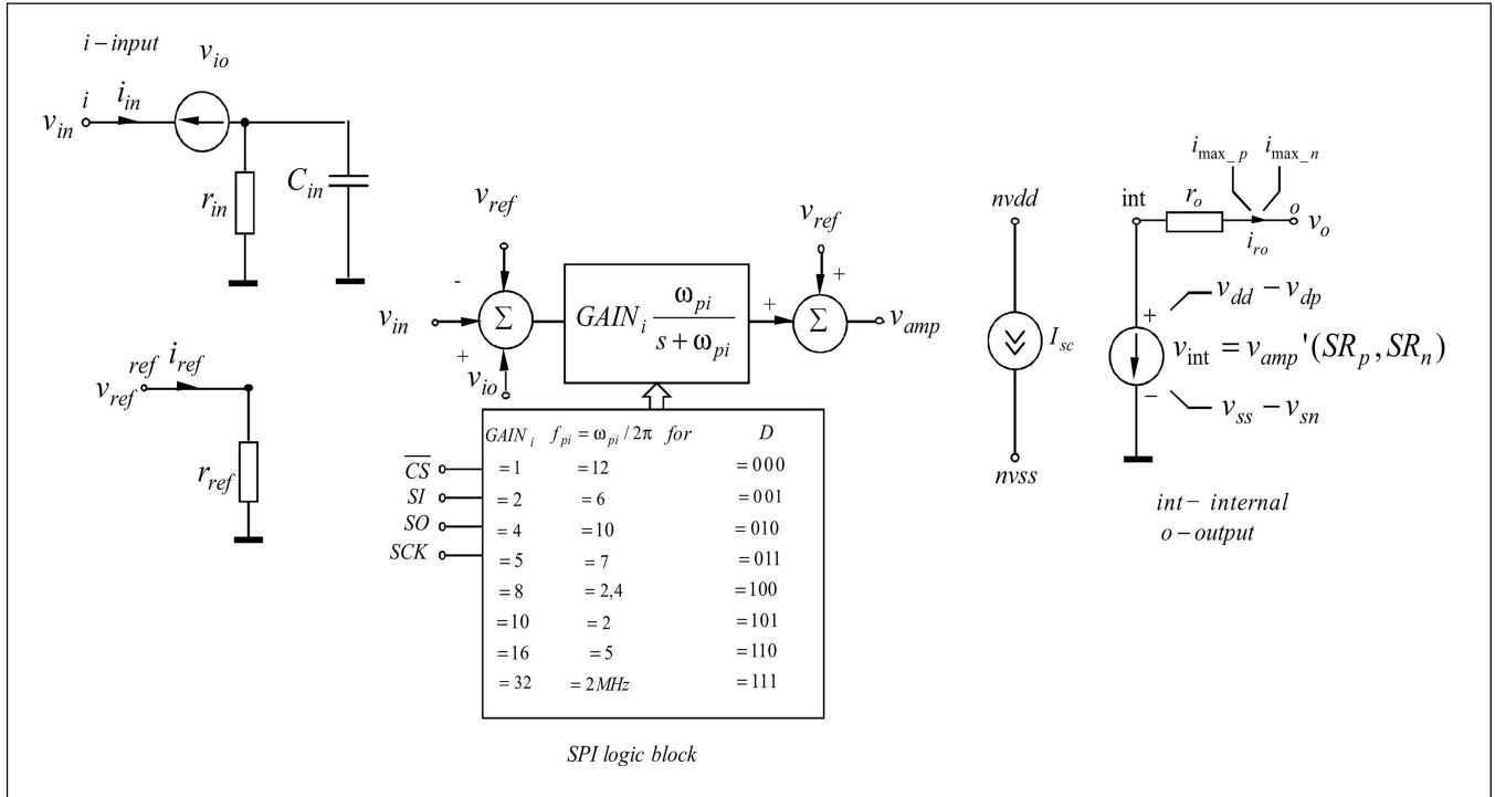
Figure 2. Circuit diagram of a one channel PGA behavioural model
