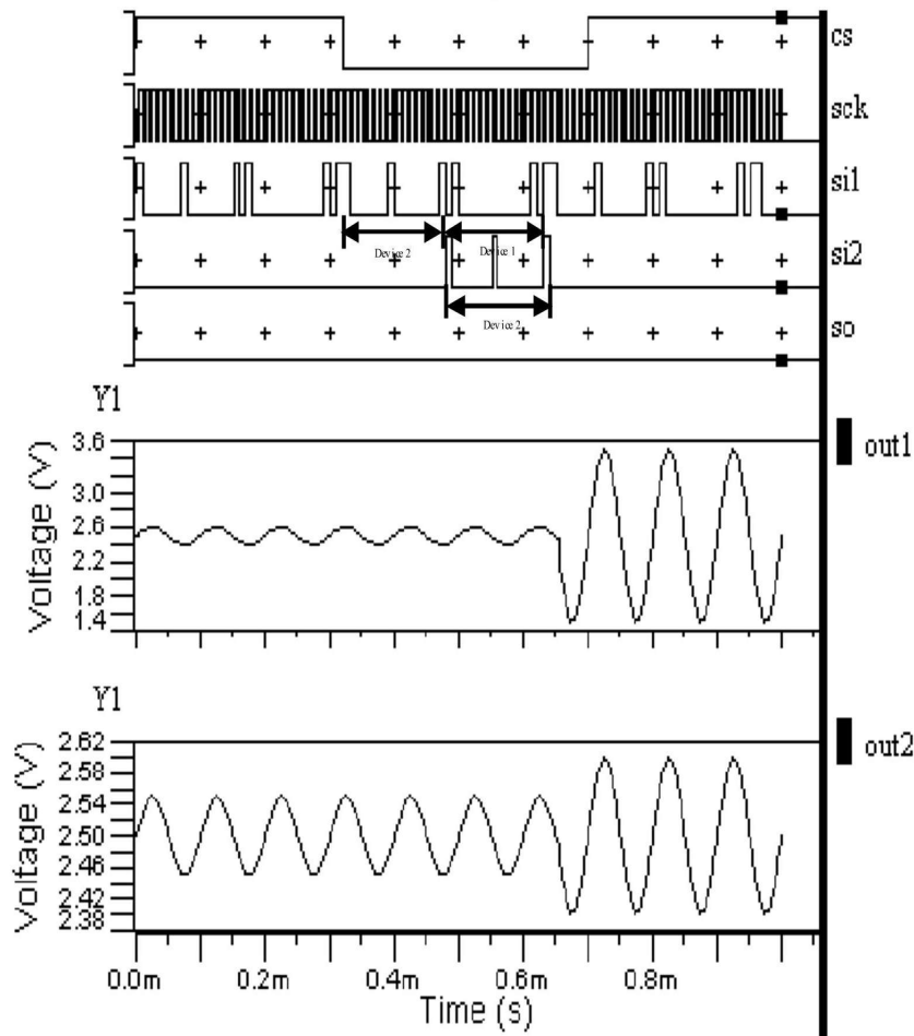
Figure 5. The simulated time domain responses for the PGA model, connected in daisy chain configuration at gain 10 and 2, respectively
