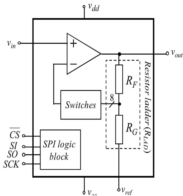
Figure 1. Monolithic PGA MCP6S21 external view [5]
