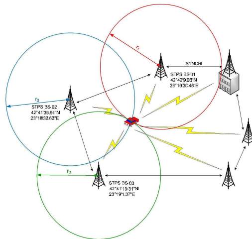
Figure 1. Synchronous terrestrial positioning system
