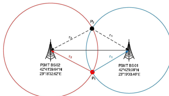
Figure 6. Determining the position of tracked mobile object only with two stationary stations
