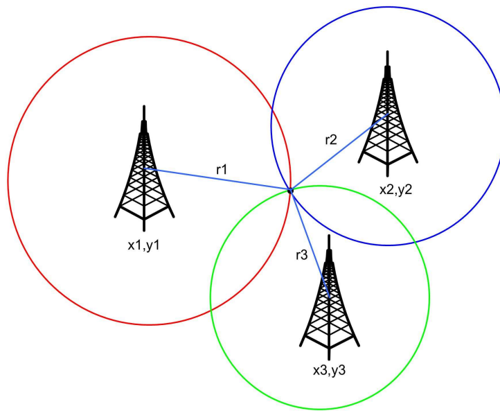
Figure 3. Determination of the coordinates of the transmitter
