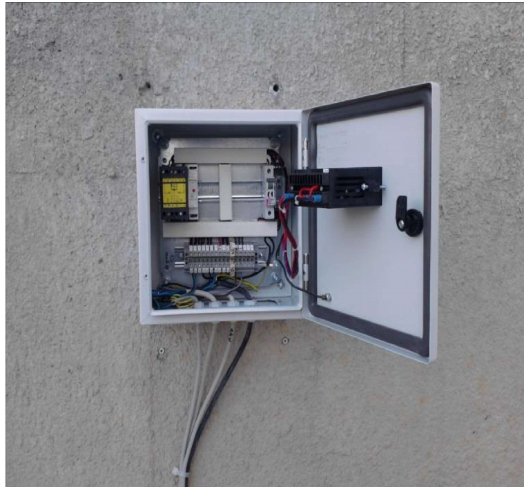
Figure 7. The cabinet with elements of the electric motor overloads protection system
