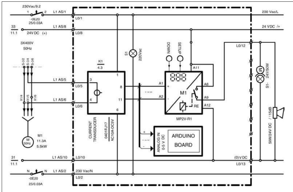
Figure 8. Electric scheme of the electric motor overload protection system with the addition of DCS node
