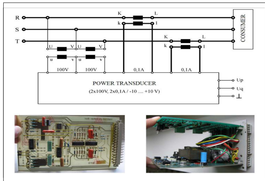
Figure 1. The principle of power transducer connection to the electric grid with the realized printed circuit boards of transducer
