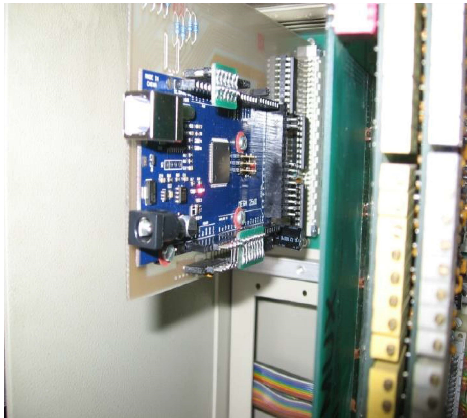
Figure 4. DCS node with an Arduino Mega board used as UMS CPU
