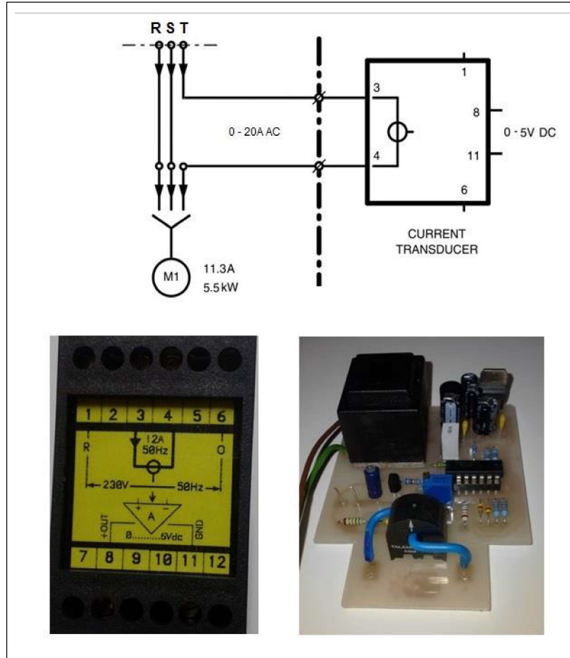
Figure 2. The principle of current transducer connection to the electric grid with the realized printed circuit boards of transducer
