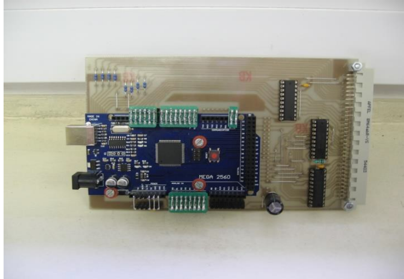
Figure 3. Arduino Mega 2560 interface board
