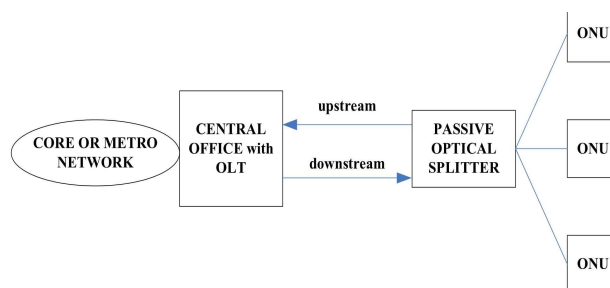
Figure 2. PON access networks
