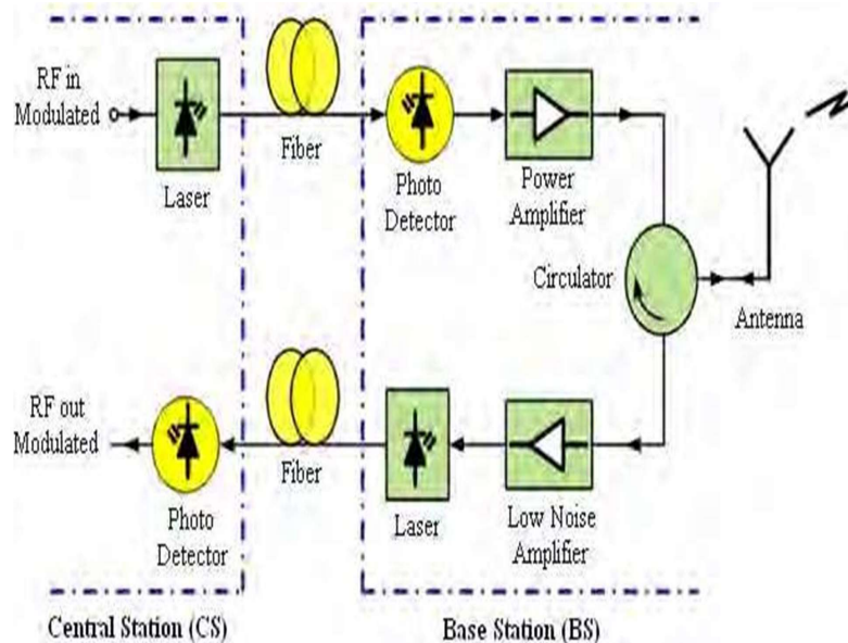
Figure 1. Basic RoF architecture
