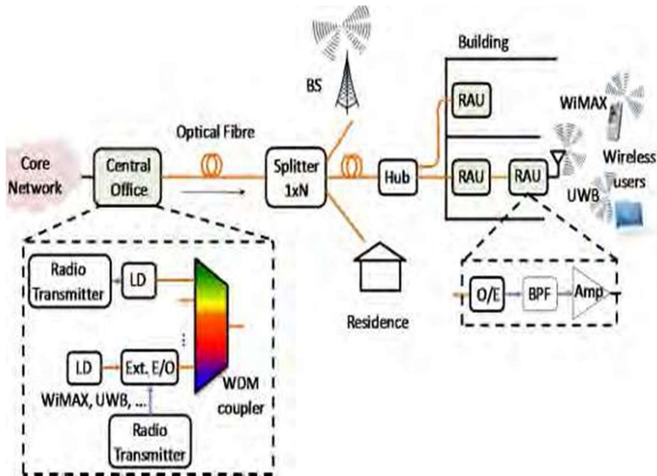
Figure 3. The complex form of the RoF technology and its central base station
