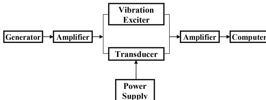
Figure 4. Block diagram of the stand for measuring vibration
