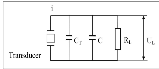
Figure 3. Equivalent replacement scheme
