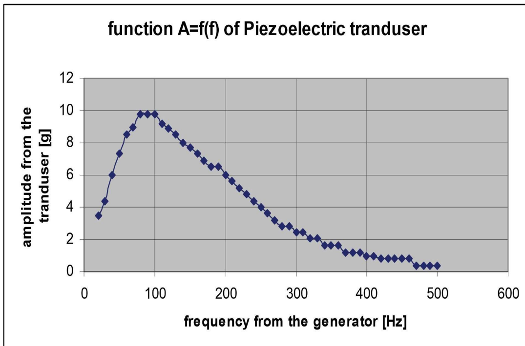
Figure 5. Function of the converting of the piezoelectric transducer from frequency of the generator
