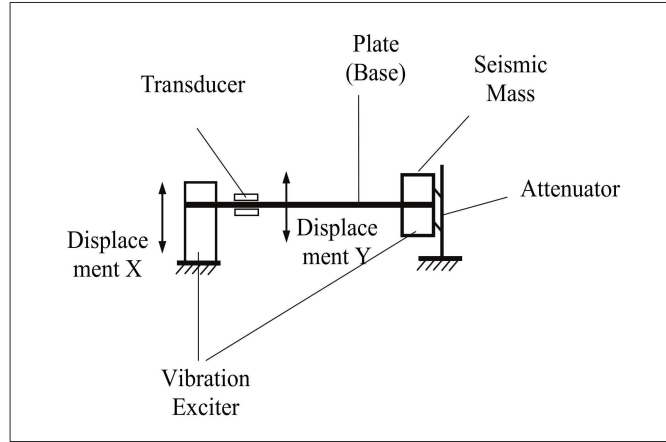
Figure 2. Stand for vibration measurements
