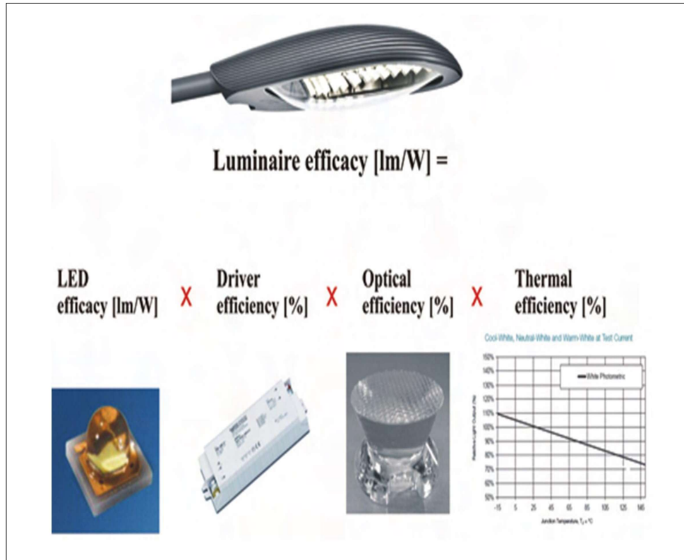
Figure 3. Luminaire efficacy [lm/W]
