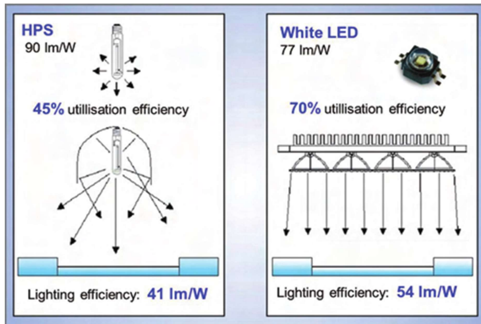
Figure 5. Utilisation efficiency - HID vs. LED in real situation
