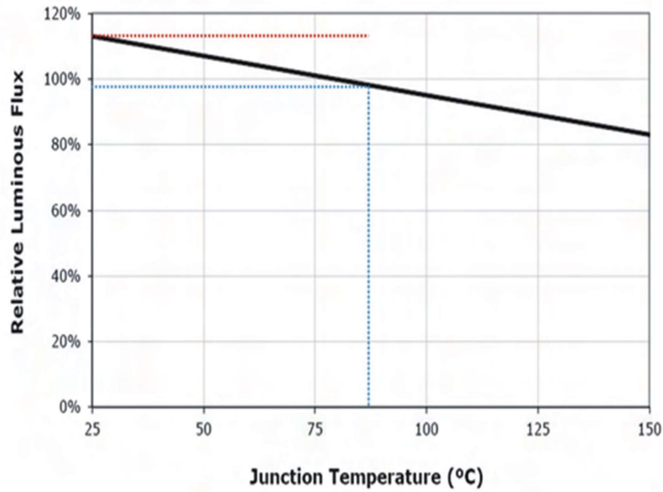
Figure 1. Relative Flux Vs. Junction Temperature (If = 350mA)
