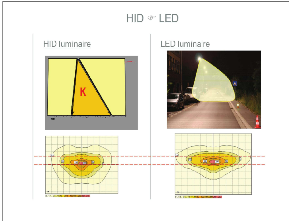
Figure 4. Utilisation efficiency HID vs. LED
