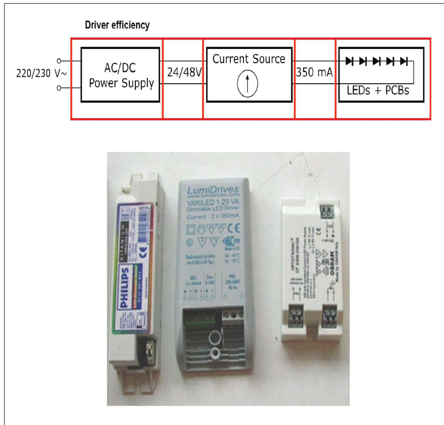
Figure 2. Typical LED circuit and the most popular drivers on the market
