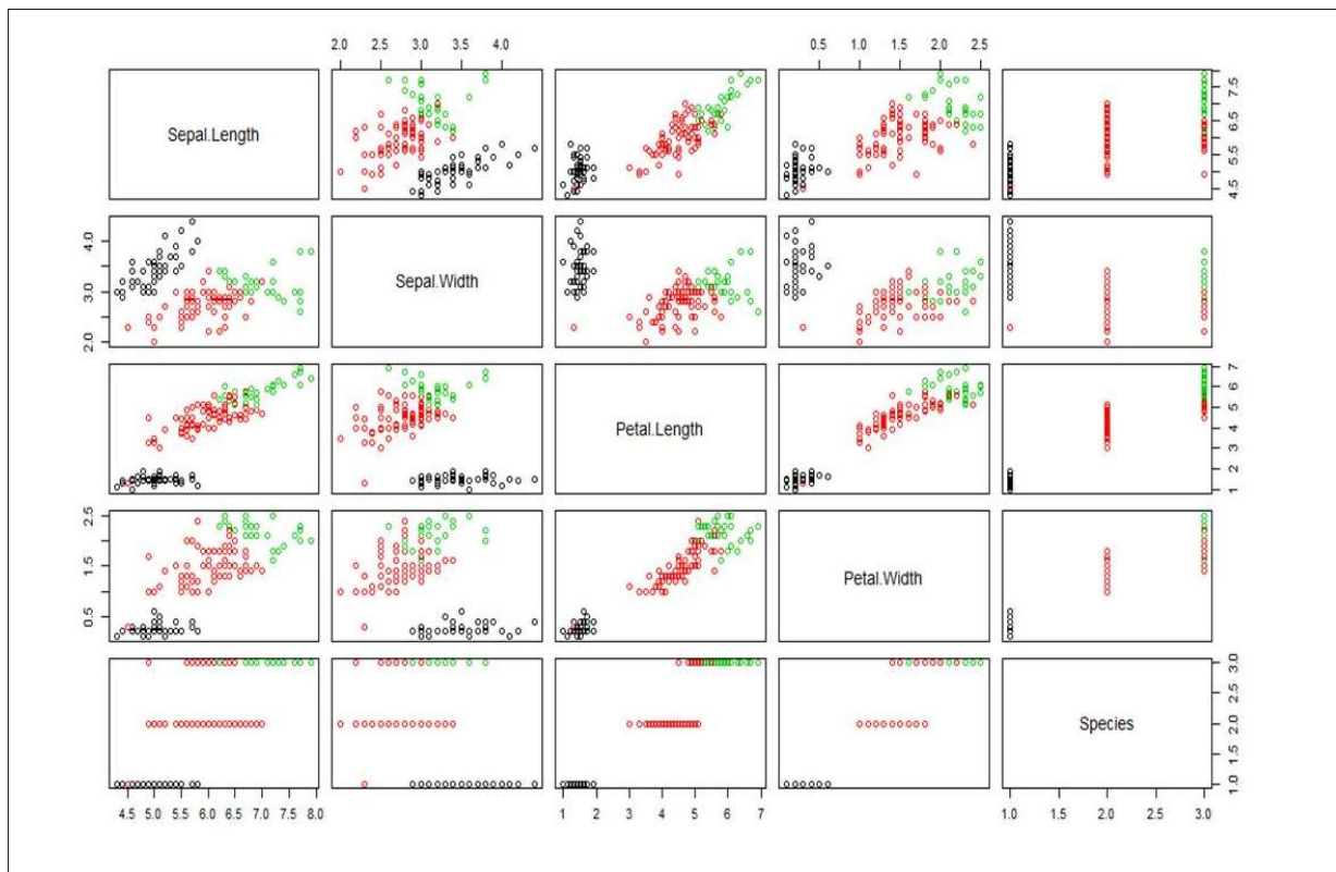
Figure 9. Scatter Plot for Hierarchical Clustering
