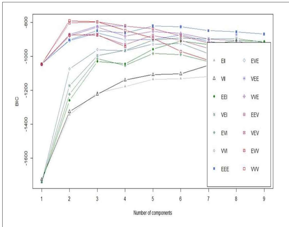
Figure 10a. BIC
