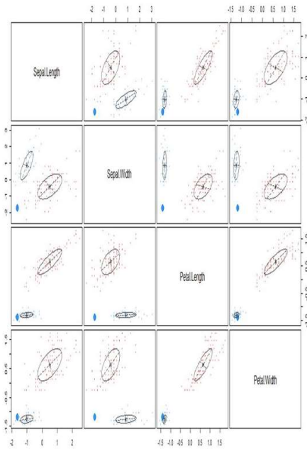
Figure 10c. Uncertainty
