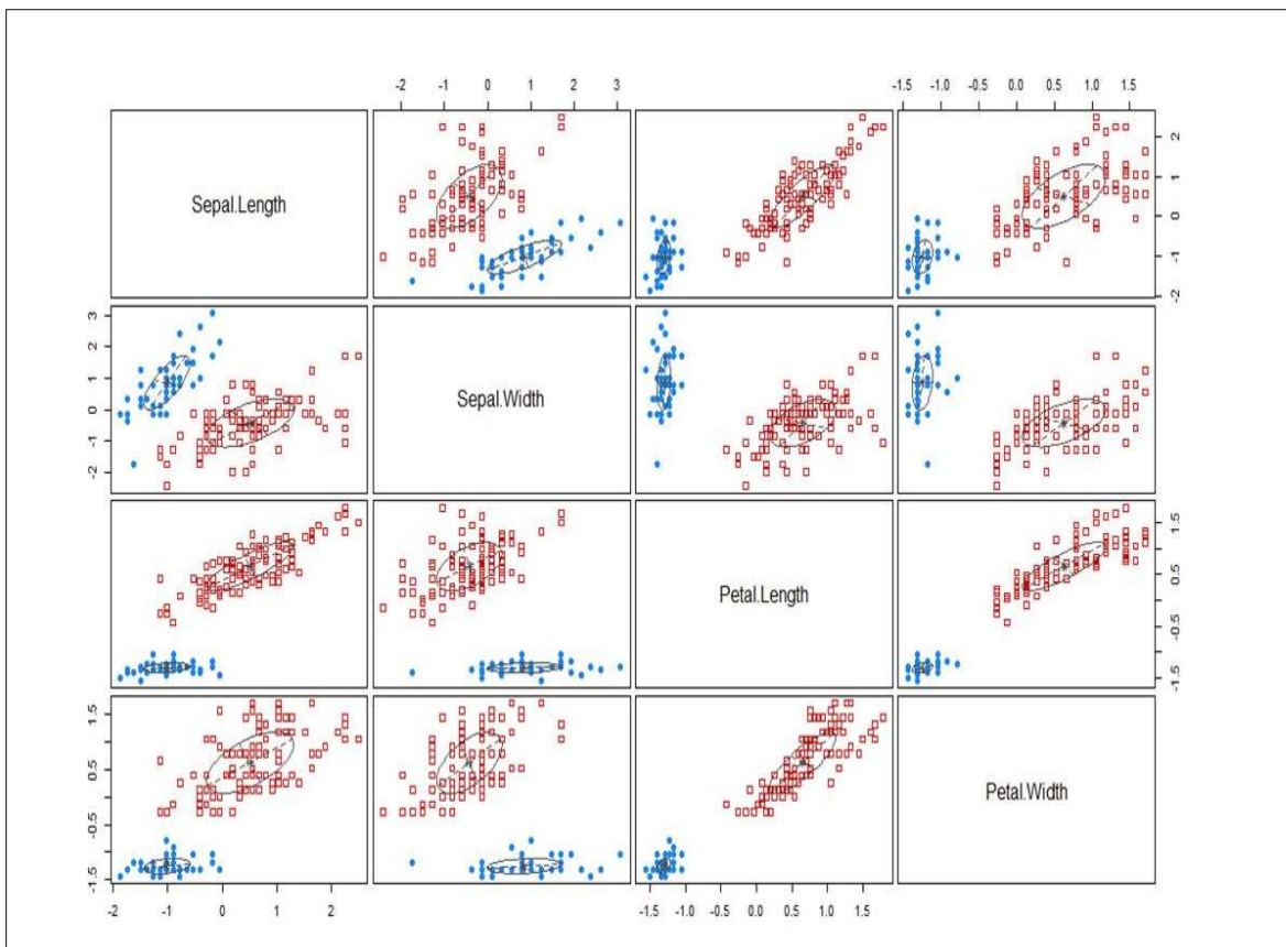
Figure 10b. Classification
