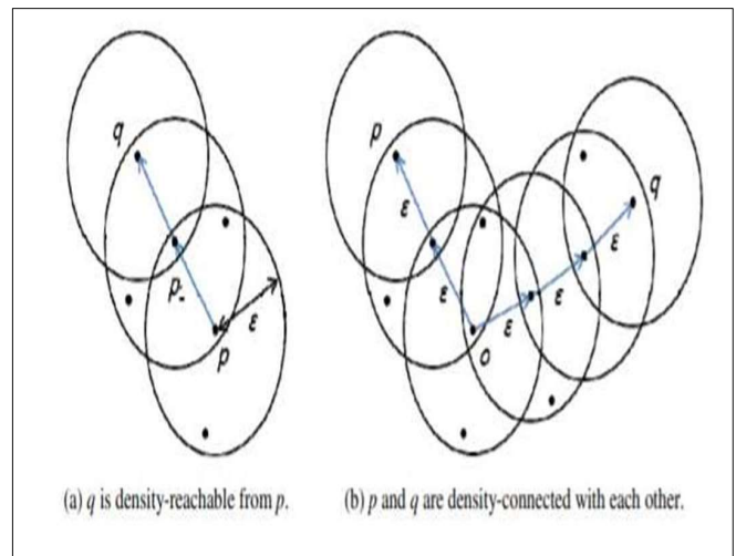
Figure 3 . Density Based Clustering
