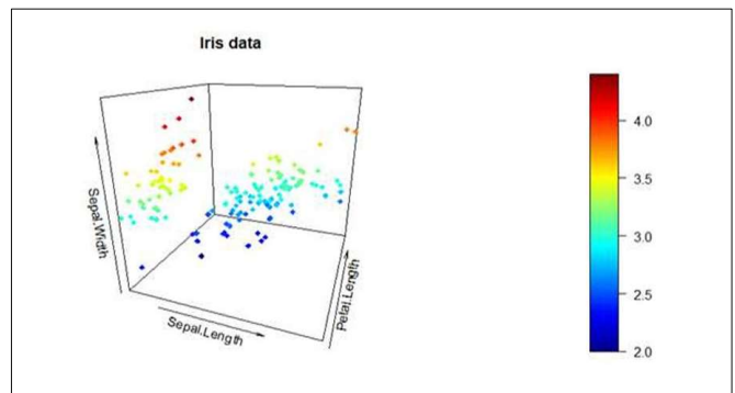
Figure 4. Iris Dataset
