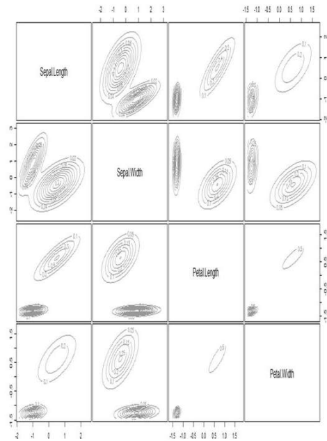
Figure 10d. Density
