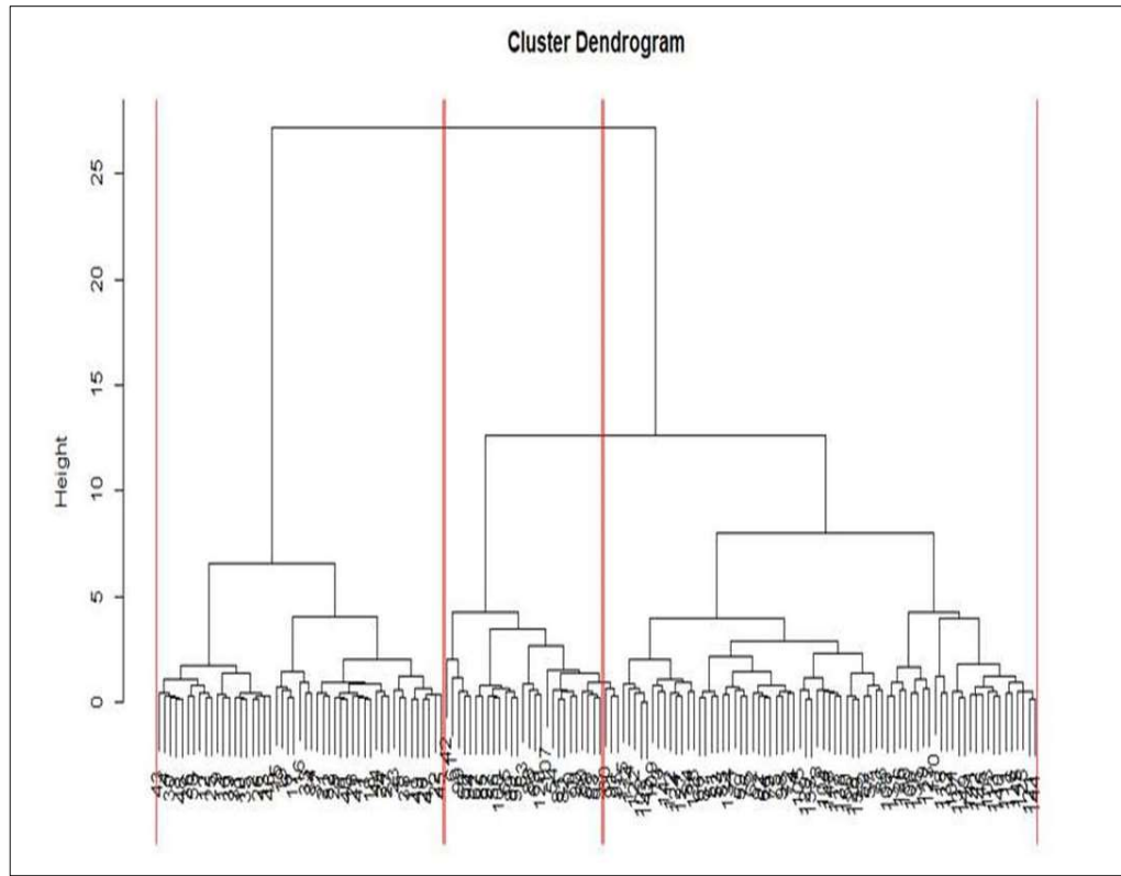
Figure 8. Dendrogram of Hierarchical Clustering
