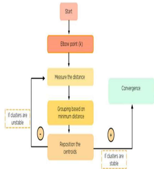
Figure 1. Steps in K-Means Algorithm
