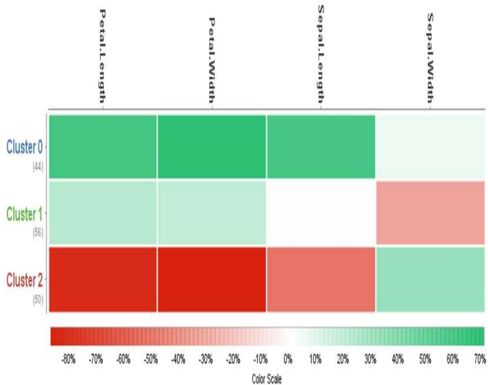
Figure 6. Heat Map
