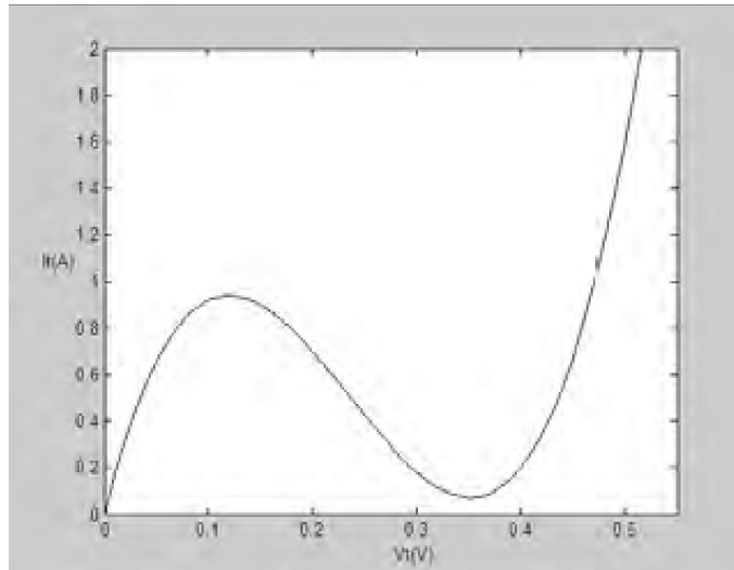
Figure 1. Current – voltage characteristic of tunnel diode
