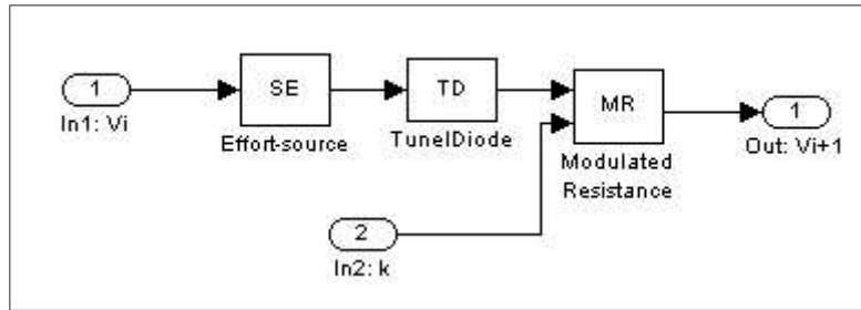
Figure 6. Bondsim model of one cascade
