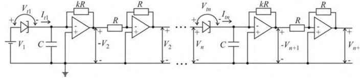
Figure 3. System of 30 cascade connected electrical circuits
