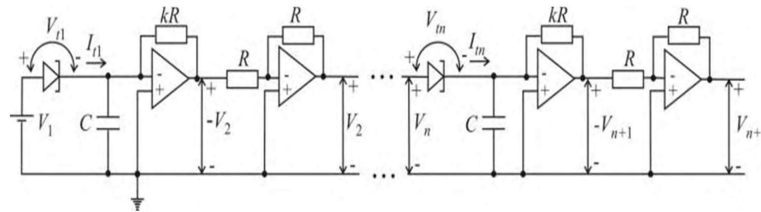
Figure 4. System of 30 cascade connected electrical circuits in the case of the quasi steady state
