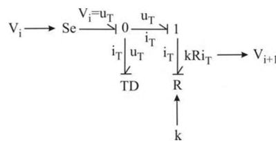
Figure 5. Bond graph model of one cascade
