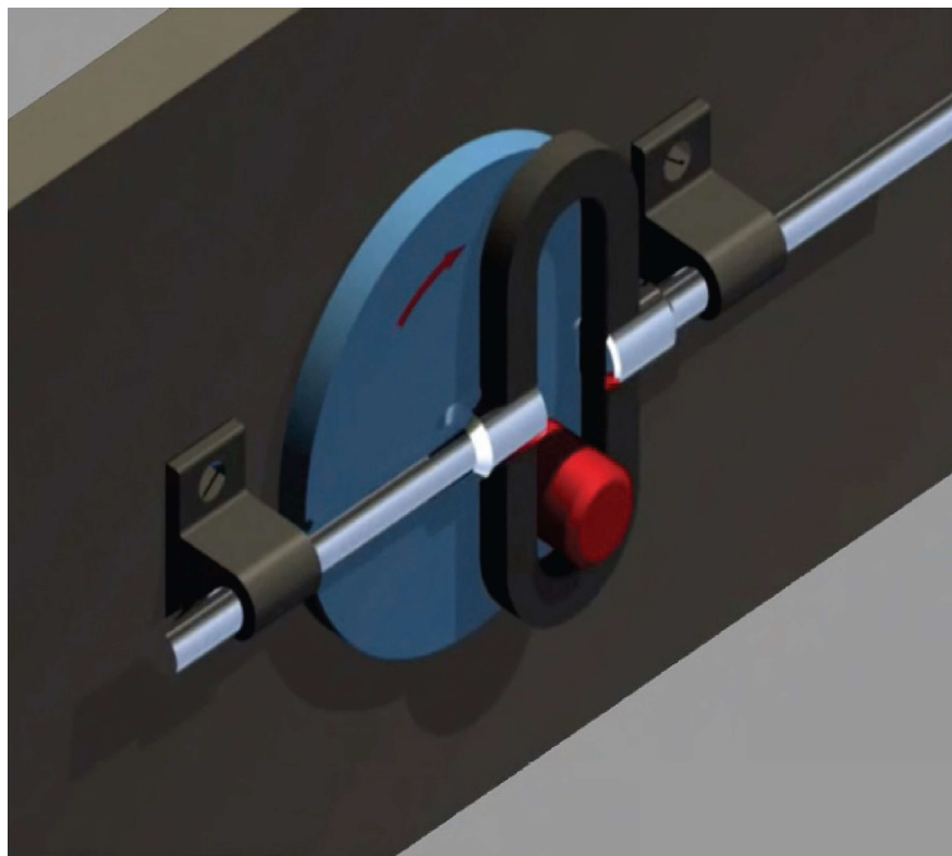
Figure 3. The crutch mechanism
