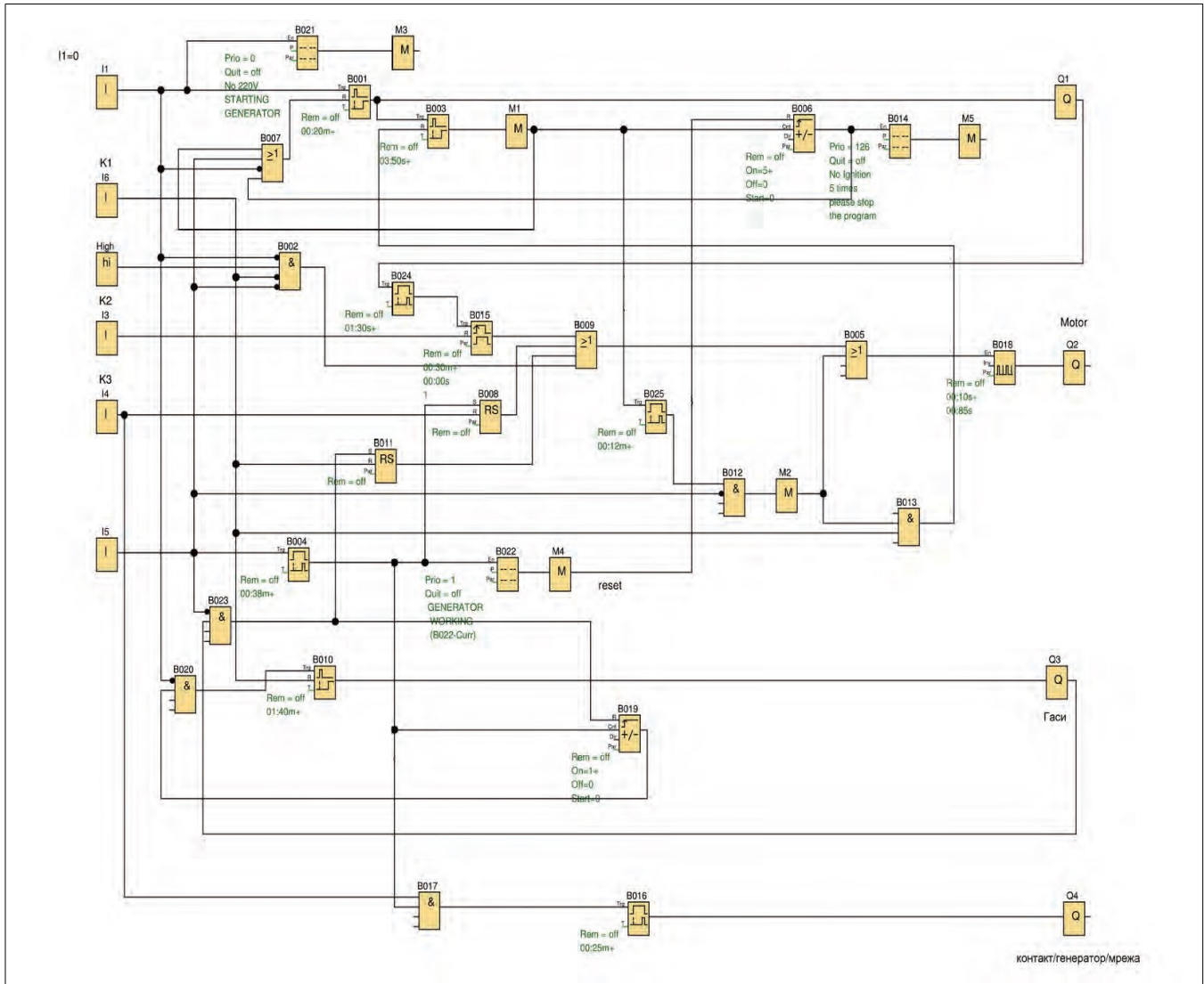
Figure 6. Block diagram of the program
