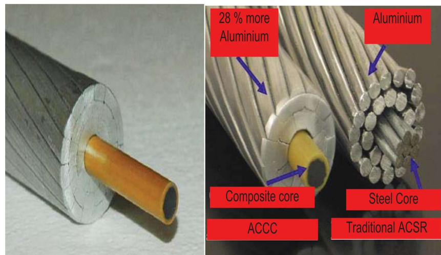
Figure 1. ACCC/TW conductor and comparison of ACCC and ACSR
