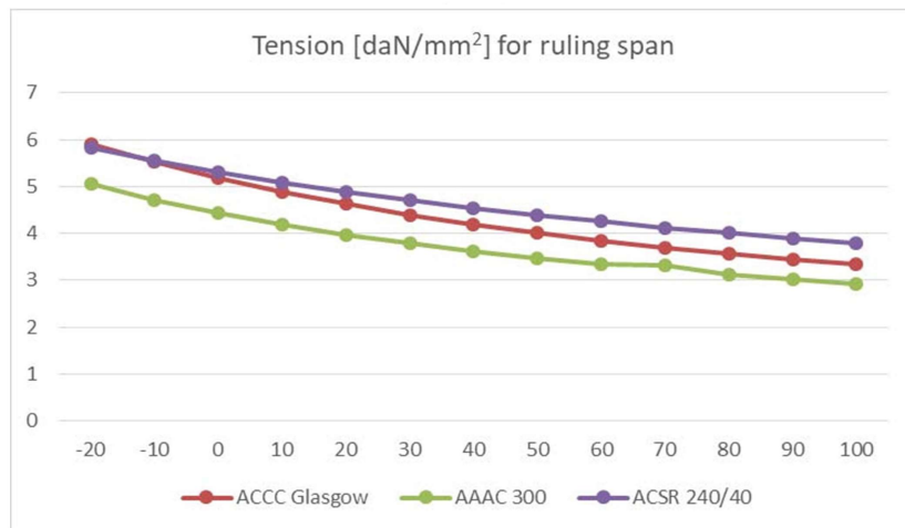
Figure 5. Tensions for ruling span for full range of temperatures -20^{\circ}\text{C} to 100^{\circ}\text{C}
