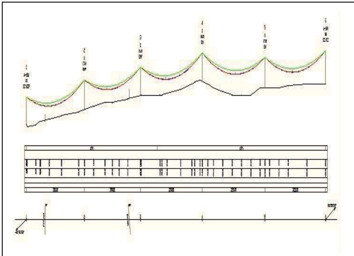
Figure 3. Tower spotting and catenary curves with each conductor
