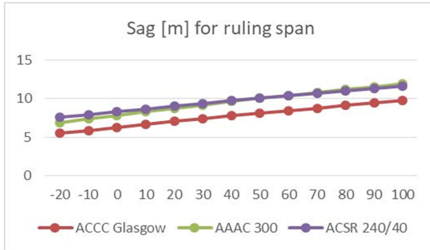
Figure 4. Sags for ruling span for full range of temperatures -20^{\circ}\text{C} to 100^{\circ}\text{C}
