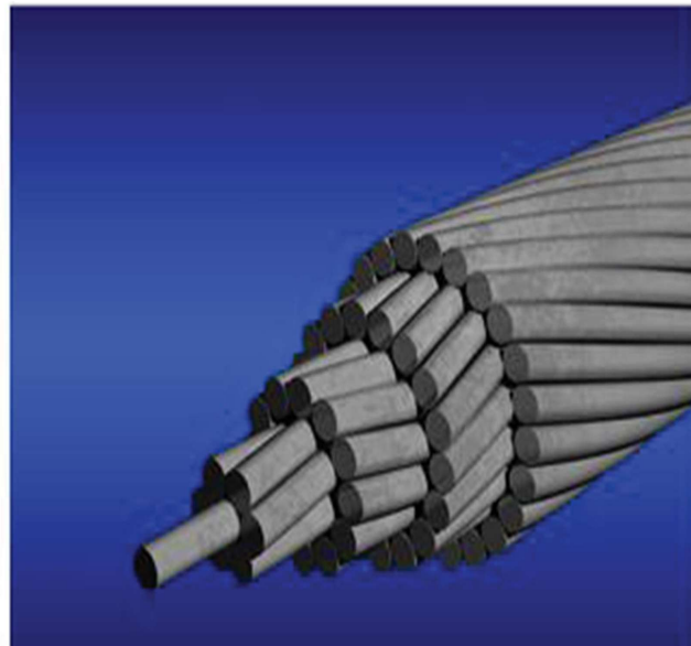
Figure 2. AAAC conductor
