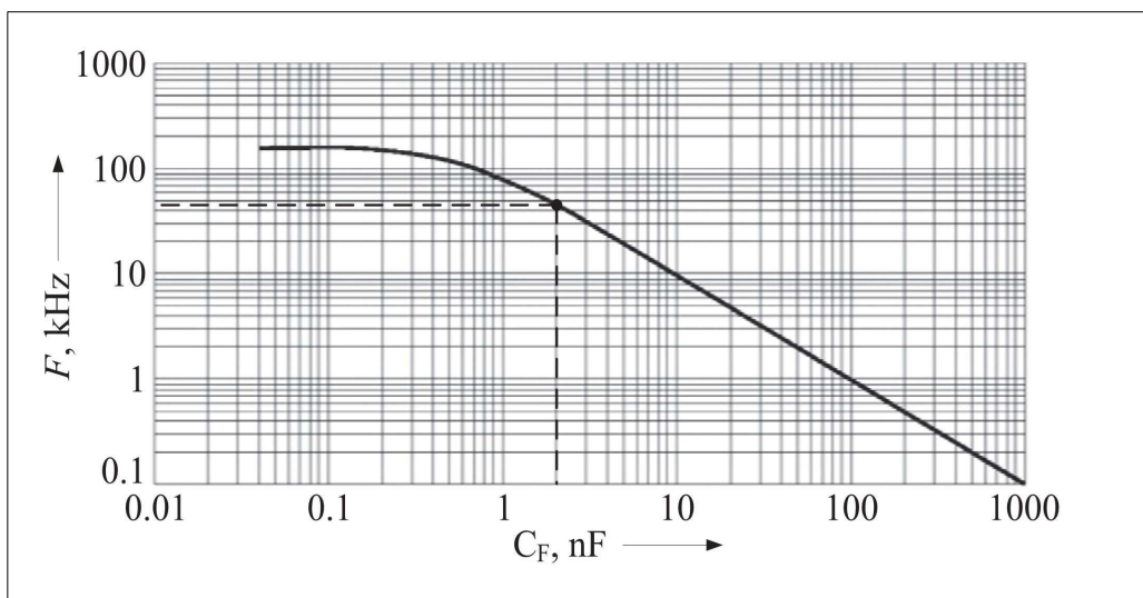
Figure 3. Dependence of the frequency of operation on the value of the F=f(CF)
