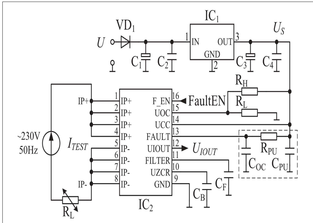
Figure 2. The circuit diagram of the developed module
