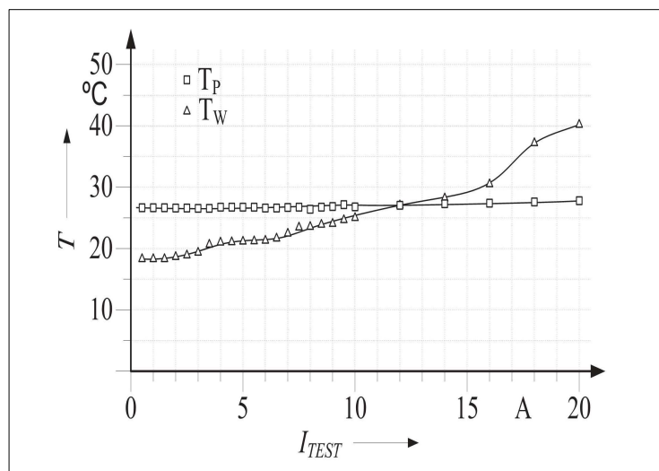
Figure 6. Graphic dependencies T_P = f(I_{TEST}) and T_W = f(I_{TEST})
