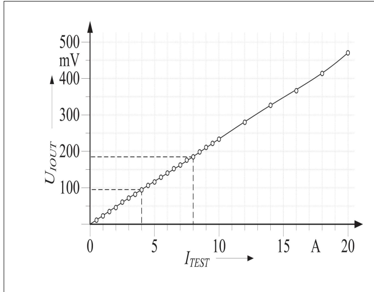
Figure 5. Experimental transmission characteristic U_{IOUT} = f(I_{TEST})
