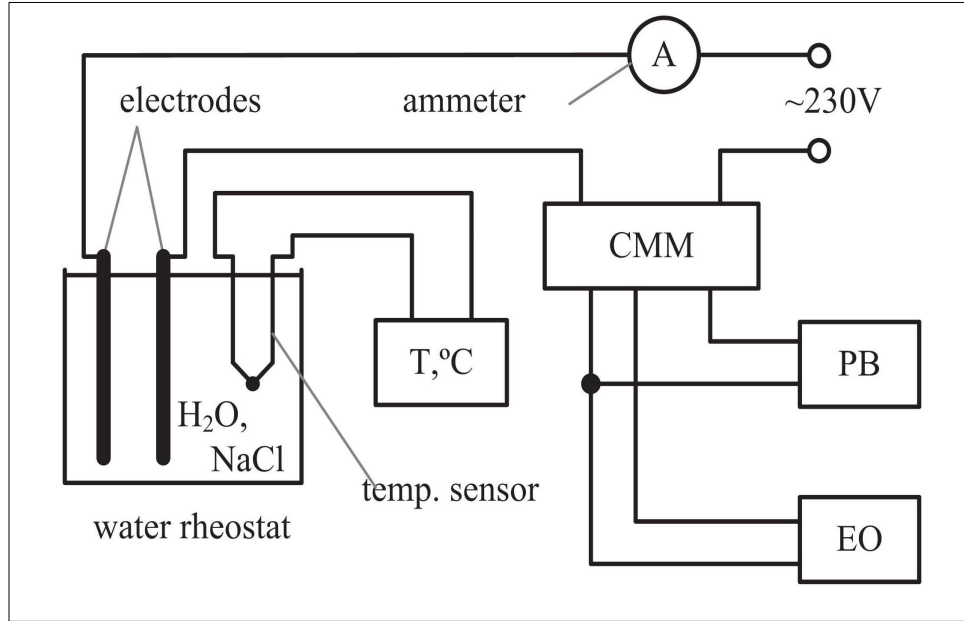
Figure 4. Schematic diagram of the experimental setup
