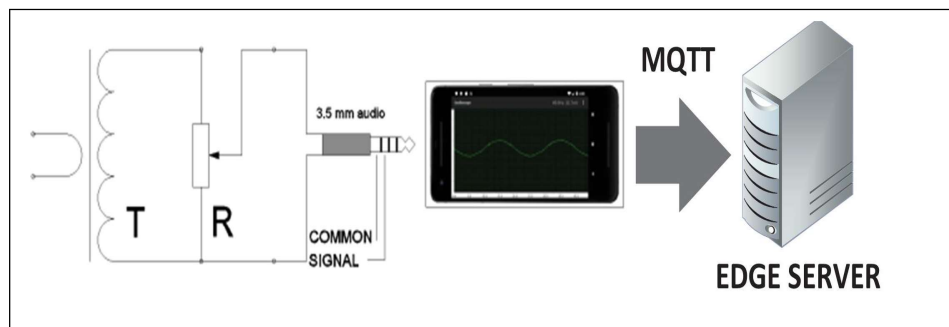
Figure 2. Android based smart measurement
