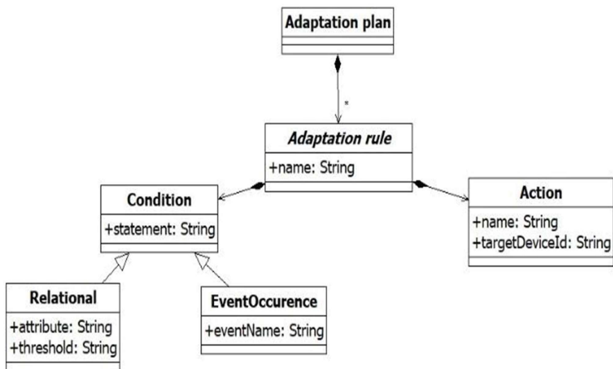
Figure 4. Adaptation plan metamodel given in UML notation
