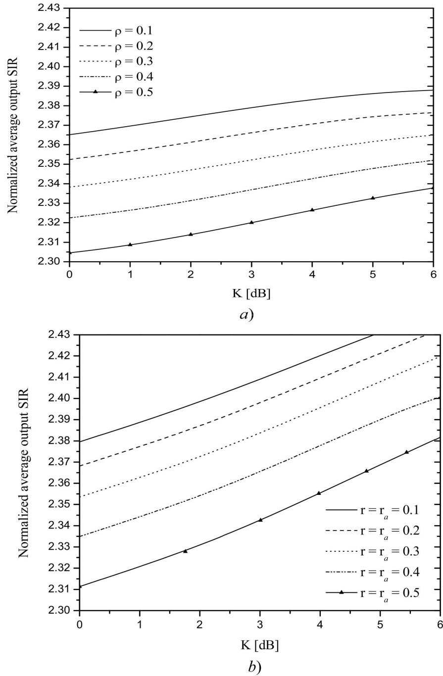
Figure 1. Average output SIR versus Rice factor for several values of correlation coefficient: a) desired signal power algorithm; b) SIR power algorithm
