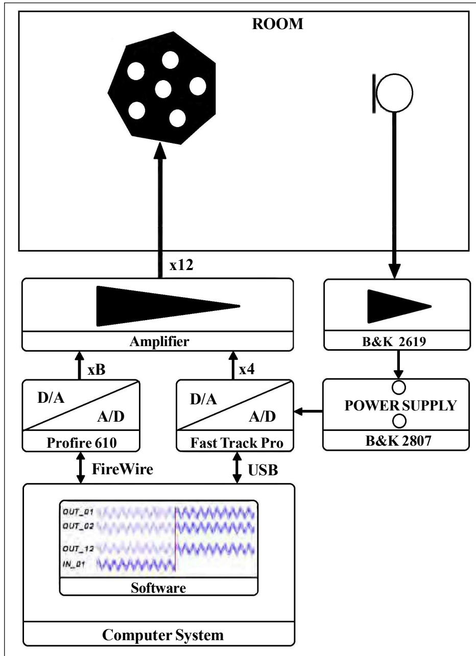
Figure 2. Measurement system
