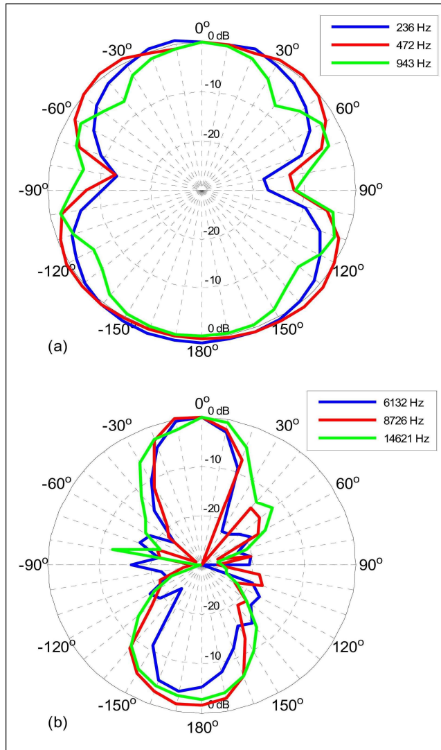
Figure 6. Radiation directivity of dodecahedral loudspeaker array with two opposite elements, one in phase and one in opposite phase on lower (a) and higher (b) frequencies
