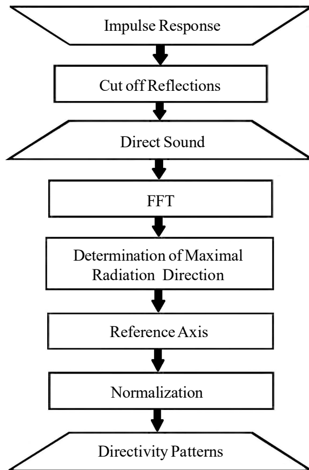
Figure 3. Impulse response processing and determination of directivity radiation pattern
