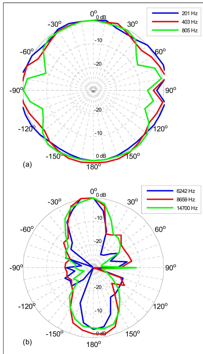
Figure 5. Radiation directivity of dodecahedral loudspeaker array with two opposite elements in phase at lower (a) and higher (b) frequencies
