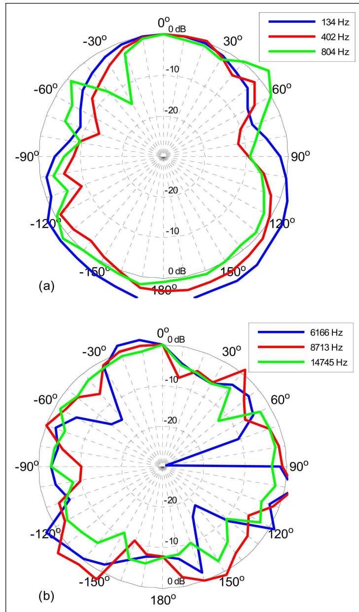
Figure 4. Radiation directivity of dodecahedral loudspeaker array with six elements in phase and six elements in opposite phase at lower (a) and higher (b) frequencies
