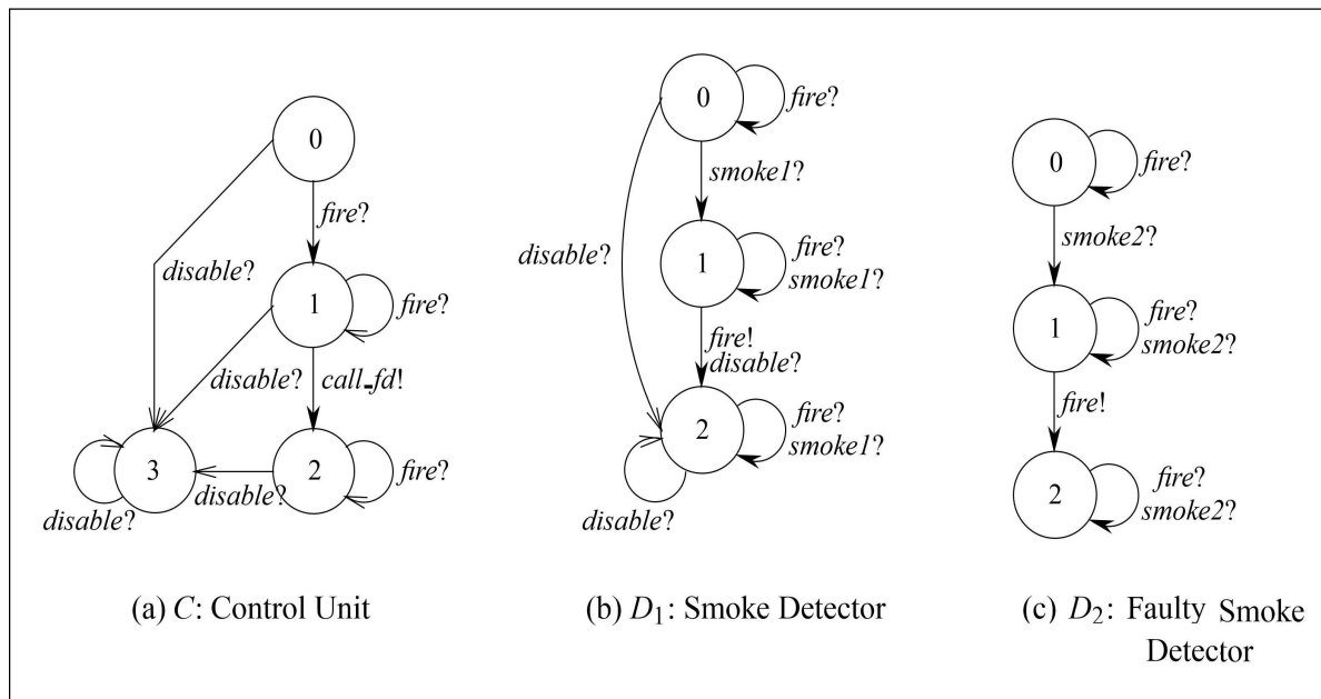
Figure 1. Sociable interface automata for a fire detection system
