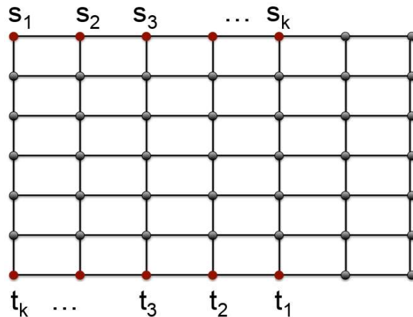
Figure 2. Integrality gap example
