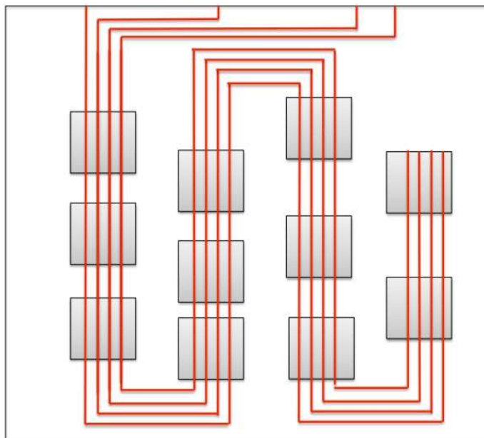
Figure 3. Traversing the boxes
